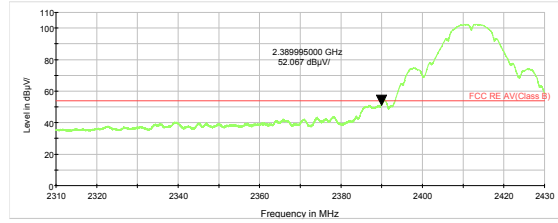
802.11b-Channel 1 Average
