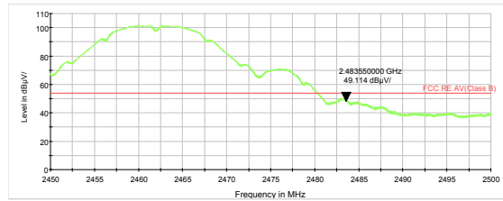
802.11b-Channel 11 Average
