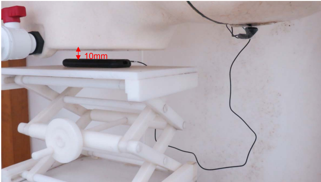
Picture 20: Back Side with Earphone, the distance from handset to the bottom of the Phantom is 10mm
