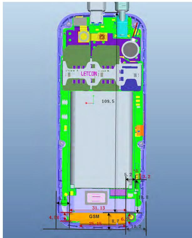
Fig.13 Antenna position of EUT
