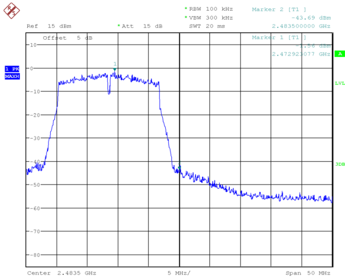
Fig.47 Band Edges (802.11g, Ch12)
