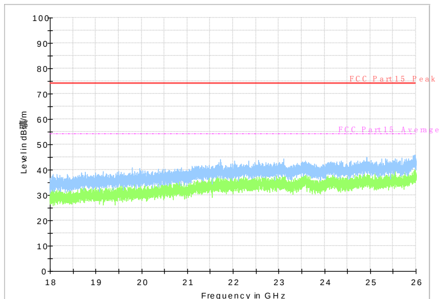
ALL Channel 18GHz~26GHz
