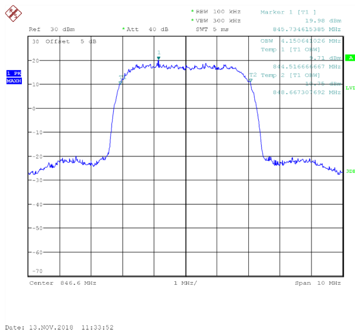
Fig.18 Channel 4233-Occupied Bandwidth (99%)
