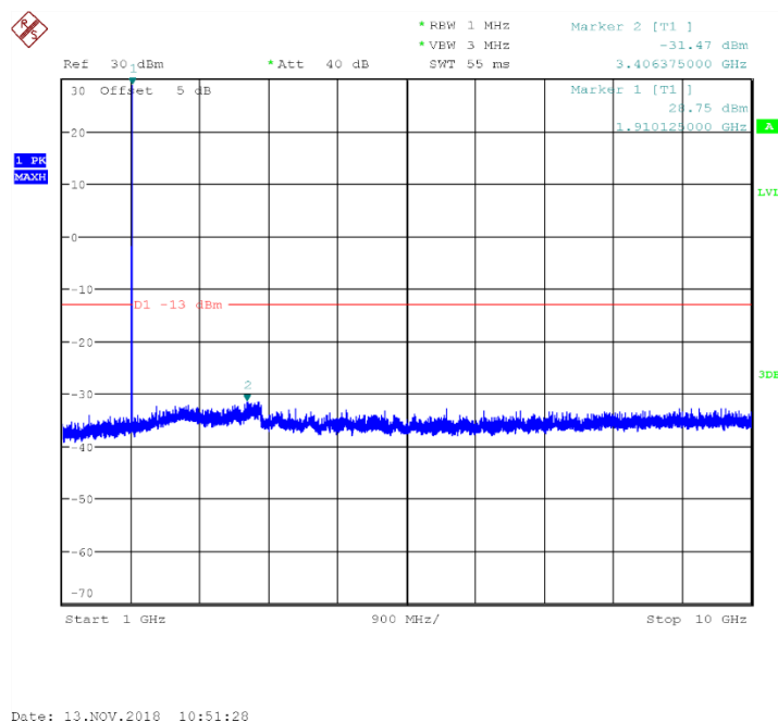
Fig.54 Channel 251: 1GHz~10GHz
