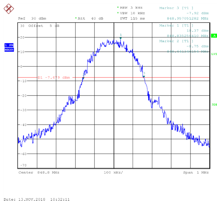
Fig.24 Channel 251- Emission Bandwidth (-26dBc BW)
