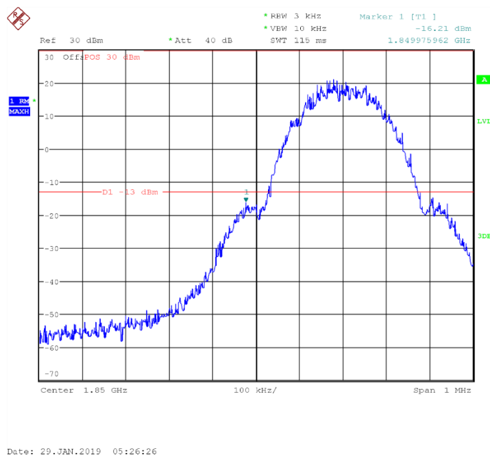
Fig.41 Channel 512- LOW BAND EDGE BLOCK
