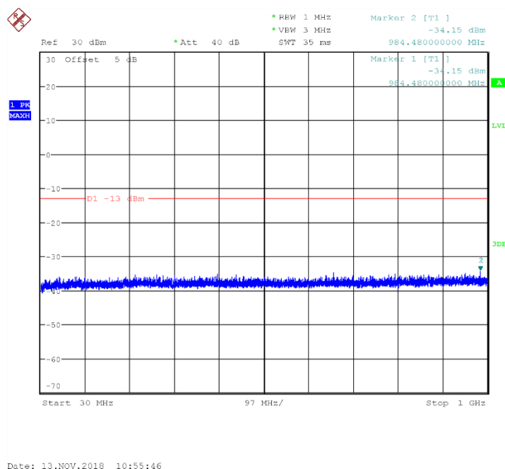
Fig.55 Channel 512: 30MHz~1GHz
