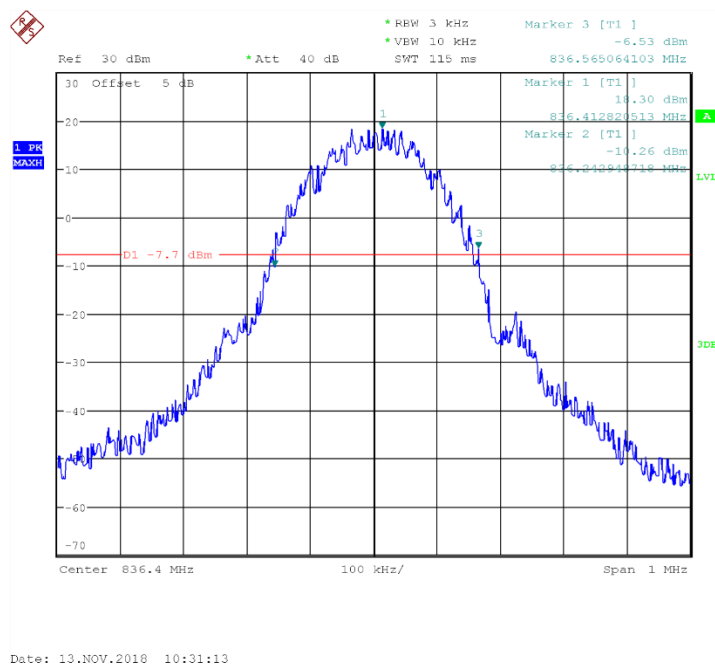
Fig.22 Channel 189- Emission Bandwidth (-26dBc BW)
