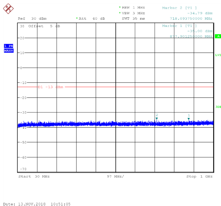
Fig.53 Channel 251: 30MHz~1GHz
