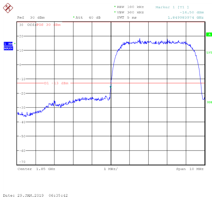
Fig.45 Channel 9262- LOW BAND EDGE BLOCK
