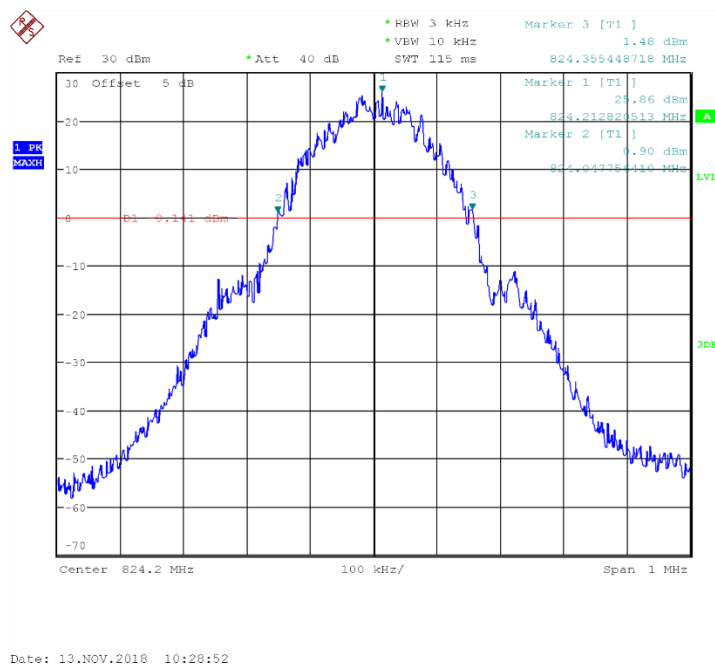
Fig.20 Channel 128- Emission Bandwidth (-26dBc BW)
