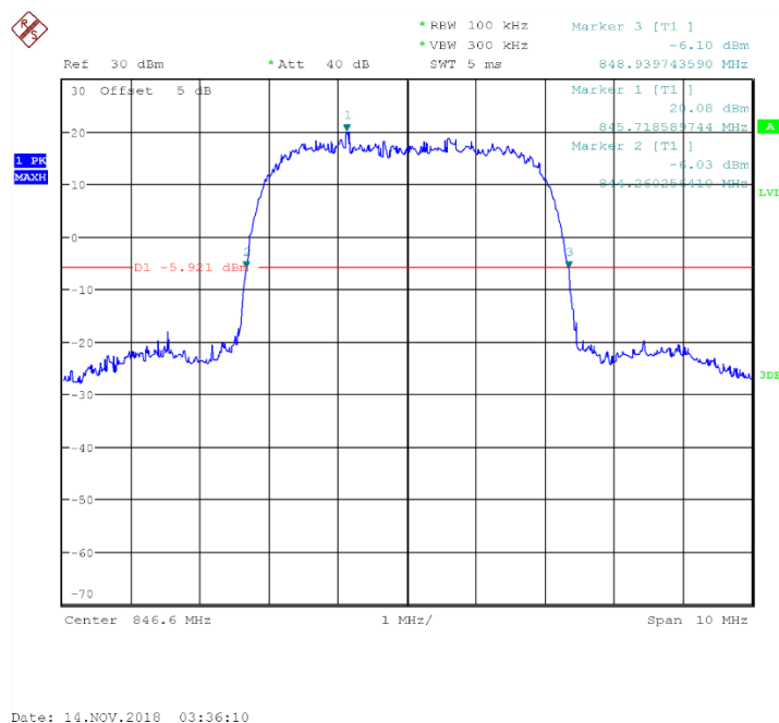
Fig.36 Channel 4233- Emission Bandwidth (-26dBc BW)
