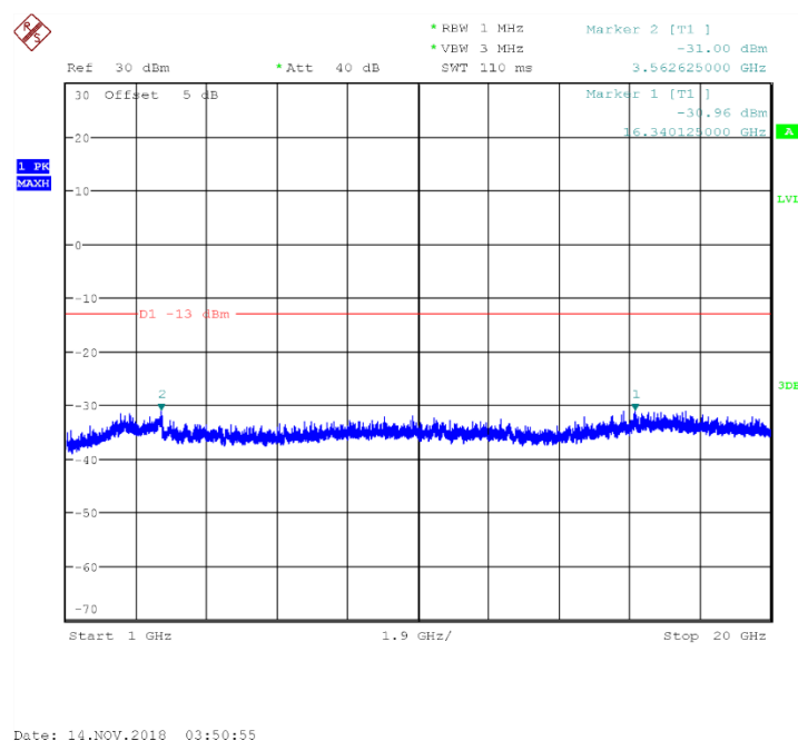
Fig.72 Channel 4233: 1GHz~20GHz
