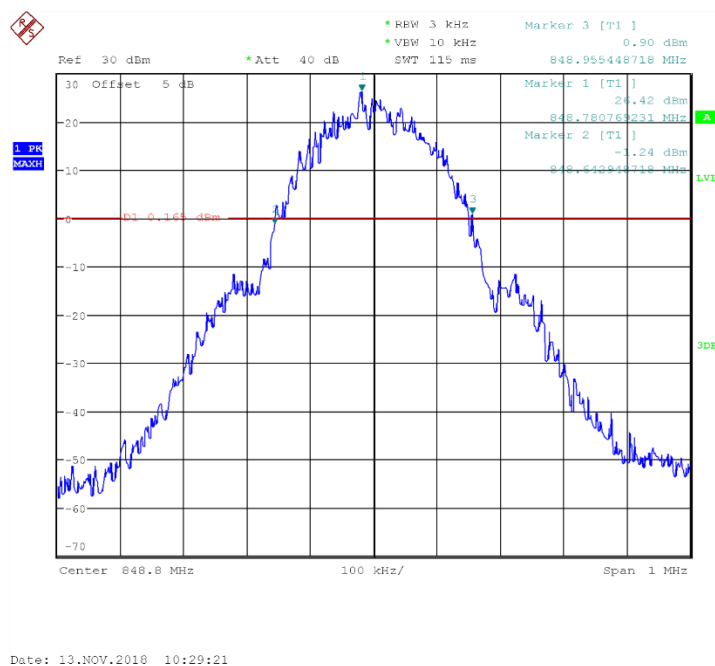
Fig.21 Channel 251- Emission Bandwidth (-26dBc BW)
