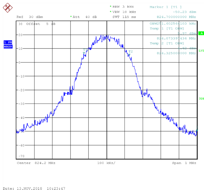
Fig.5 Channel 128-Occupied Bandwidth (99%)
