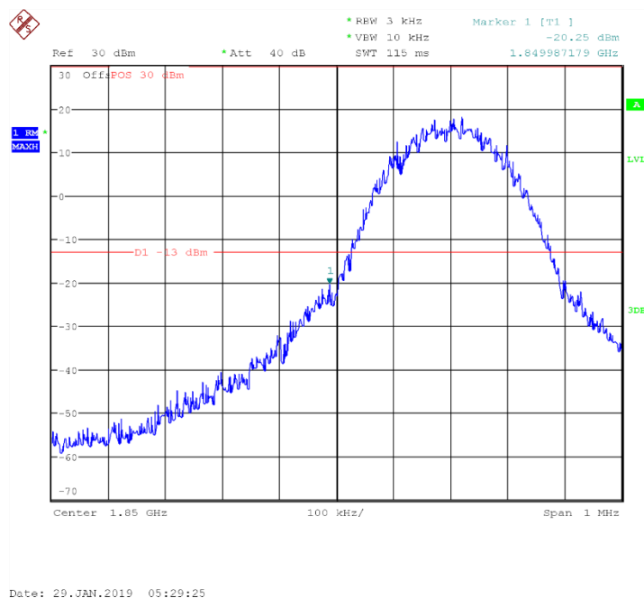
Fig.43 Channel 512- LOW BAND EDGE BLOCK
