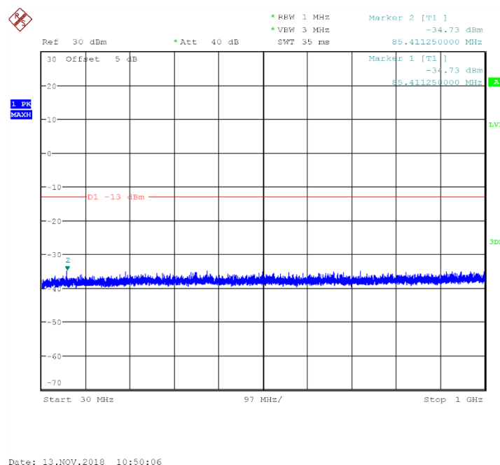
Fig.49 Channel 128: 30MHz~1GHz
