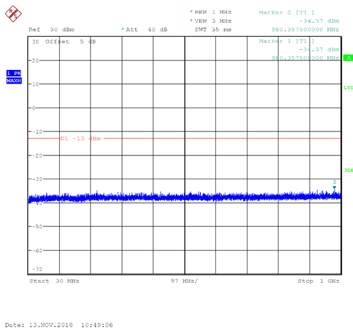
Fig.51 Channel 189: 30MHz~1GHz
