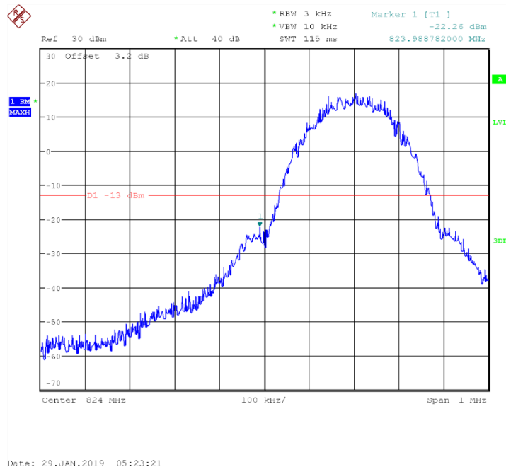
Fig.39 Channel 128- LOW BAND EDGE BLOCK
