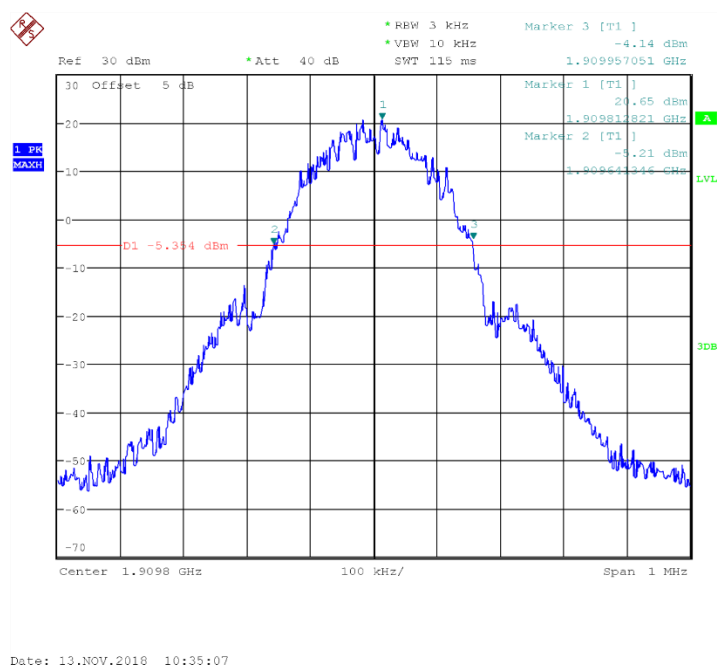
Fig.27 Channel 810- Emission Bandwidth (-26dBc BW)
