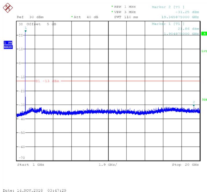
Fig.66 Channel 9538: 1GHz~20GHz
