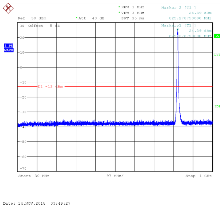
Fig.67 Channel 4132: 30MHz~1GHz
