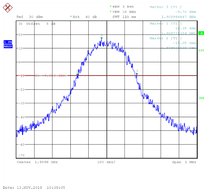
Fig.30 Channel 810- Emission Bandwidth (-26dBc BW)
