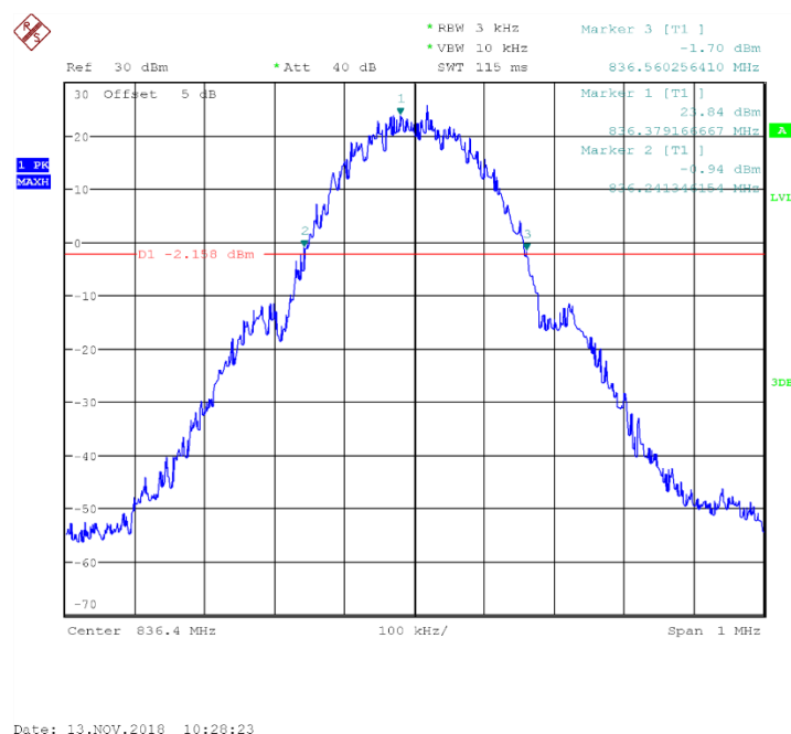
Fig.19 Channel 189- Emission Bandwidth (-26dBc BW)
