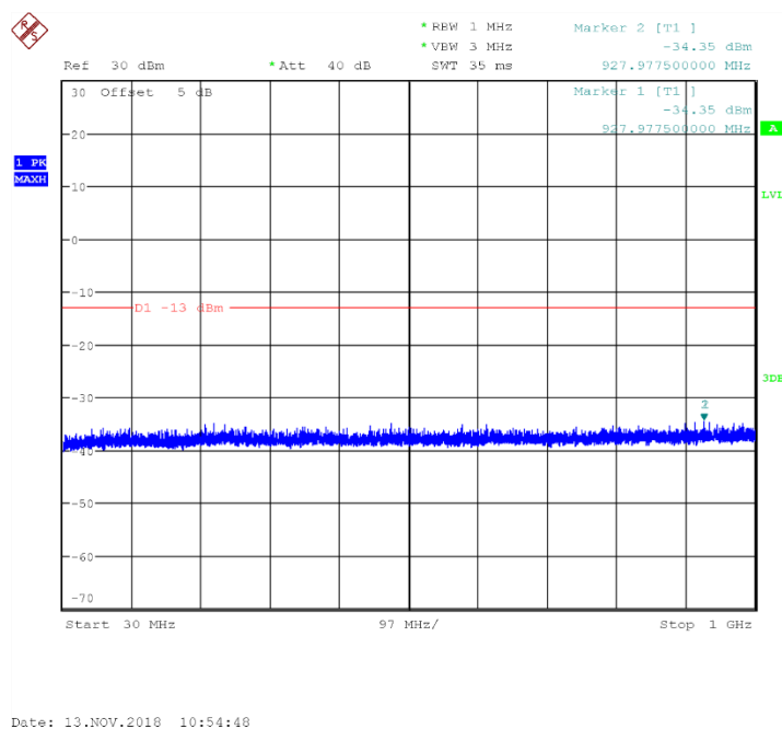
Fig.57 Channel 661: 30MHz~1GHz
