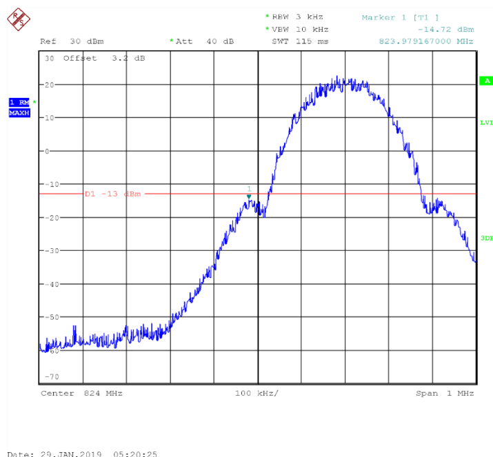
Fig.37 Channel 128- LOW BAND EDGE BLOCK
