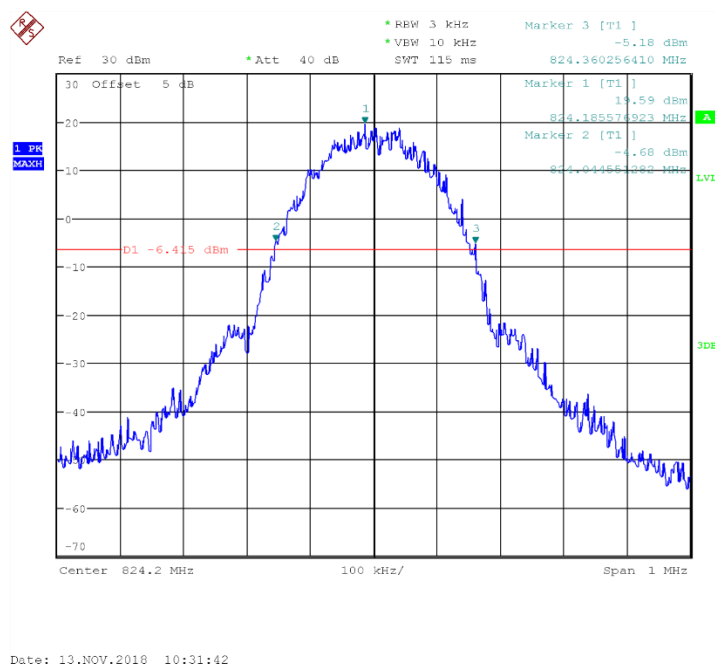
Fig.23 Channel 128- Emission Bandwidth (-26dBc BW)
