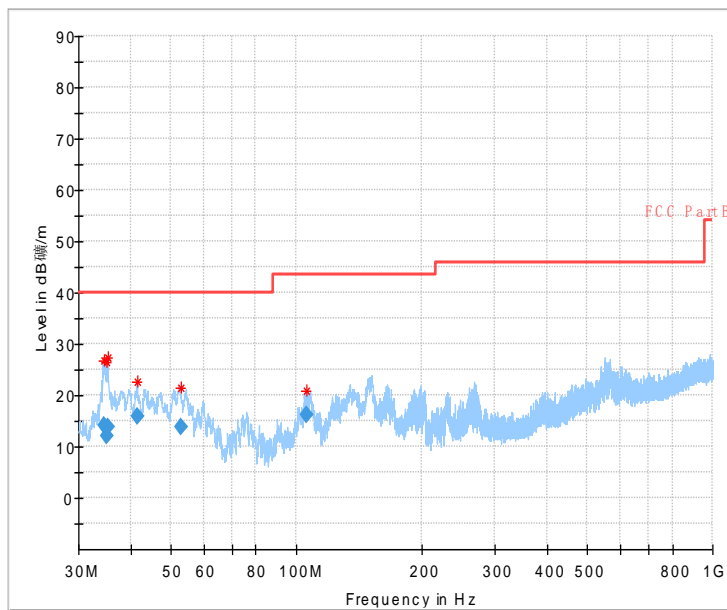
Fig.51 Radiated Spurious Emission (802.11g,Ch11,30MHz~1GHz)
