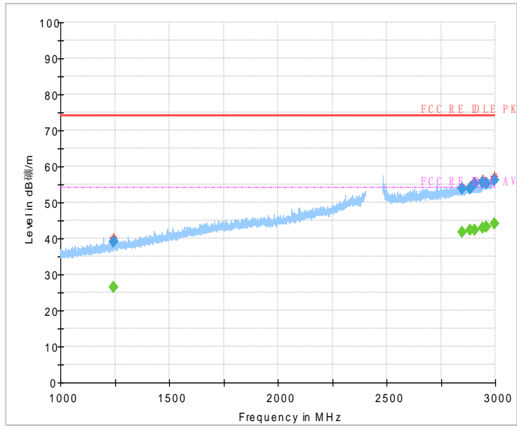
Fig.52 Radiated Spurious Emission (802.11g,Ch11,1GHz~3GHz)
