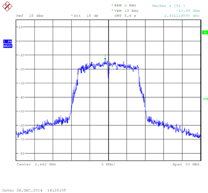
Fig.6 Power Spectral Density (802.1g,Ch11)
