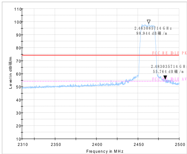
Fig.55 Radiated emission (Power): 802.11n, high channel
