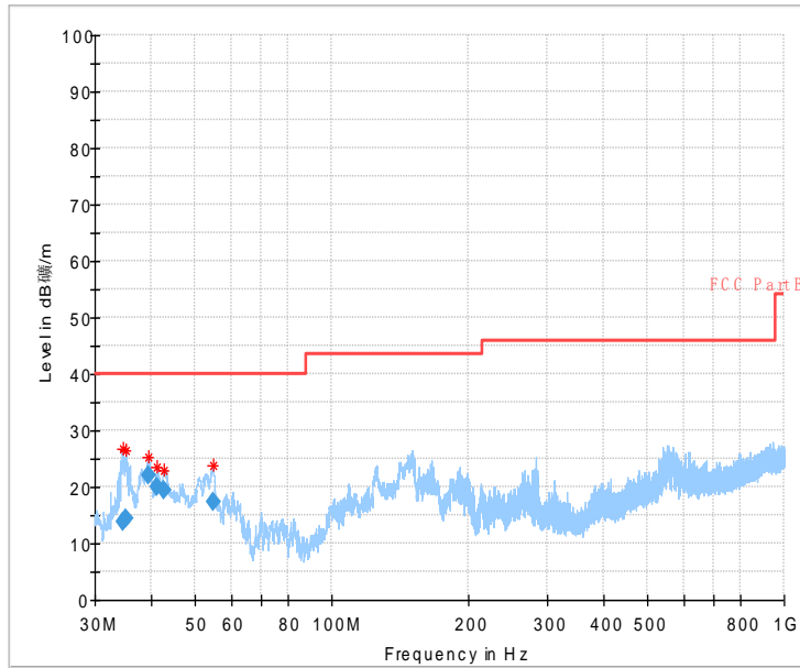
Fig.46 Radiated Spurious Emission (802.11b,Ch1,30MHz~1GHz)
