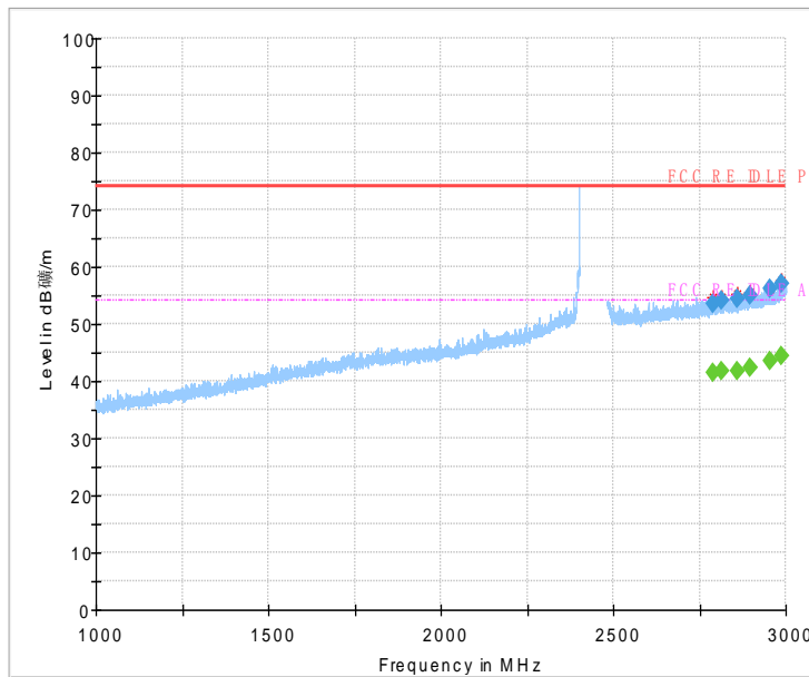
Fig.57 Radiated Spurious Emission (802.11 n-20MHz,Ch1,1GHz~3GHz)
