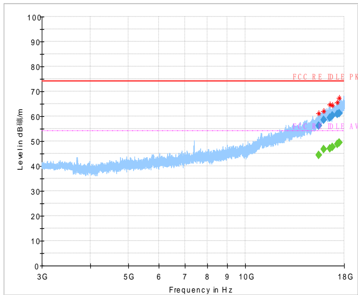
Fig.53 Radiated Spurious Emission (802.11g,Ch11,3GHz~18GHz)
