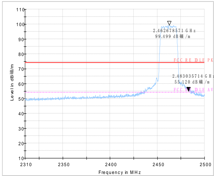
Fig.50 Radiated emission (Power): 802.11g, high channel
