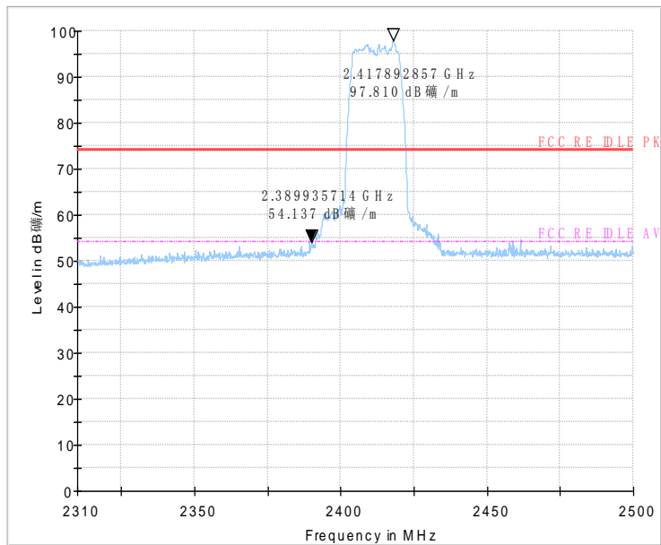
Fig.54 Radiated emission (Power): 802.11n, low channel
