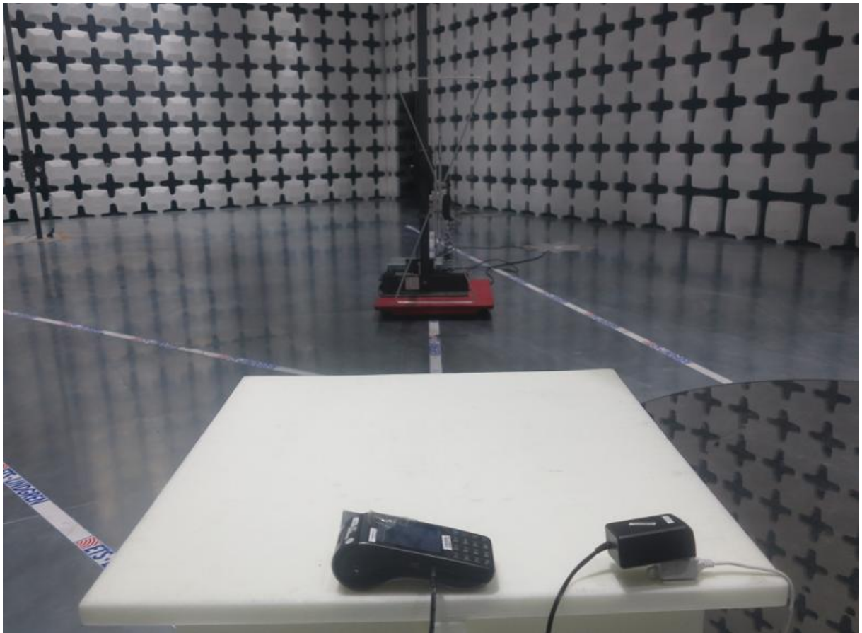
Picture C-2: Field Strength Measurements (Above 30MHz)
