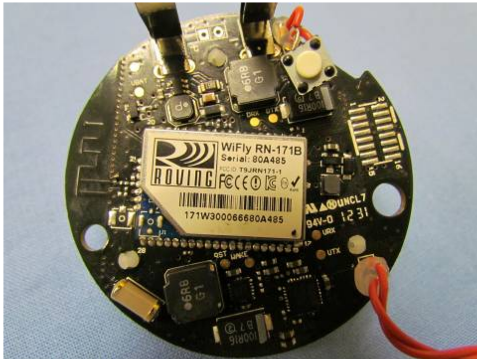
Board top view
