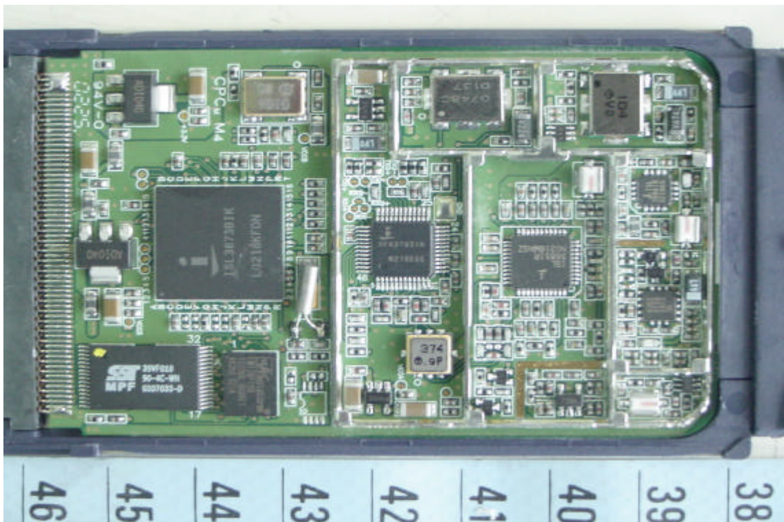
29. Component View of RF Module PCB
