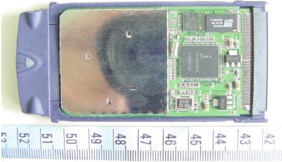
29. Component View of RF Module PCB
