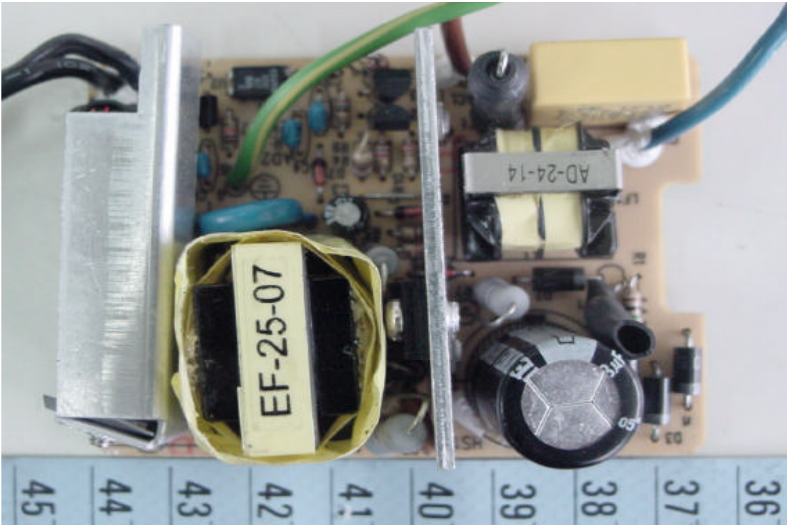
34. Component View of Adaptor's PCB
