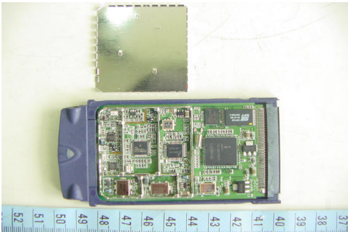
27. Internal View of RF Module
