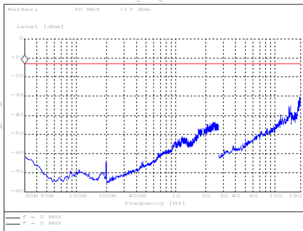
S661HT for GPRS mode
