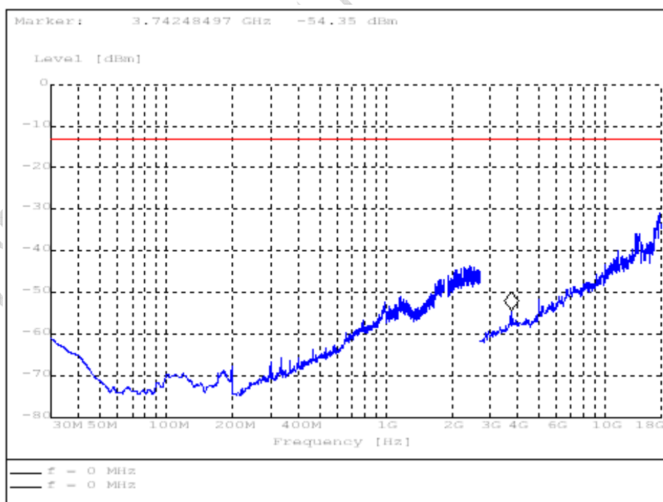
S661HF for GSM mode
