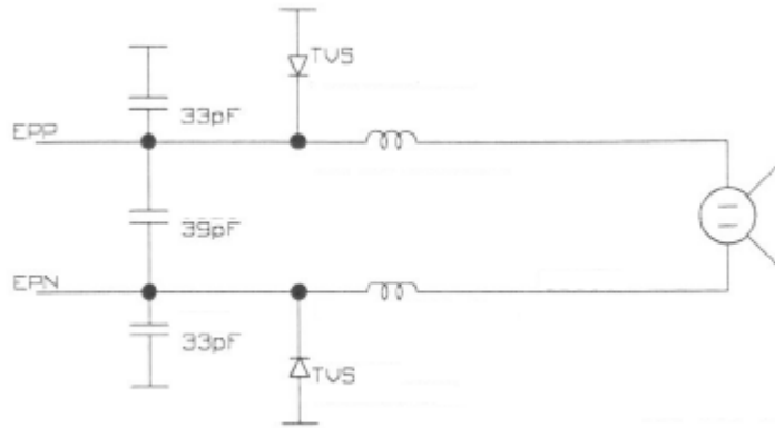
Figure 10: Example of earphone implementation
