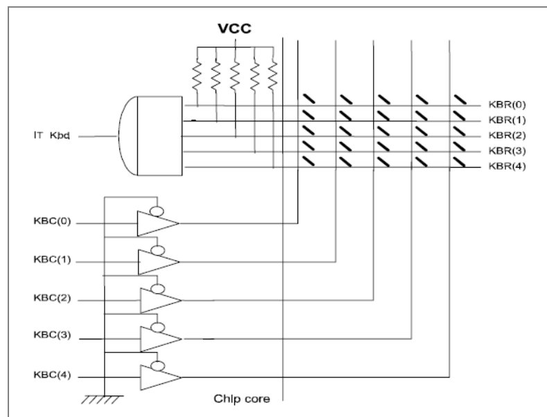
Figure 11: Keyboard Implementation Diagram
