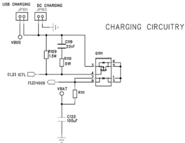
Figure 5: Charging Circuit Diagram Example
