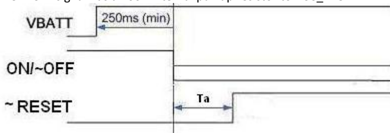
Figure 6. Reset Timing
