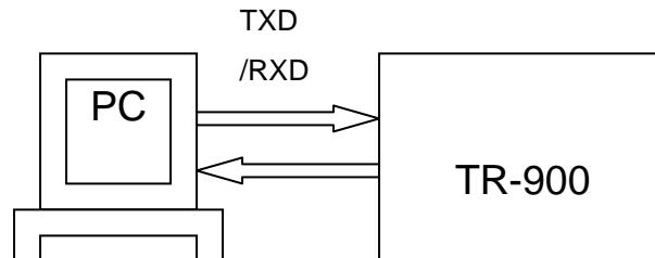
Figure 7: Interfacing with UART
