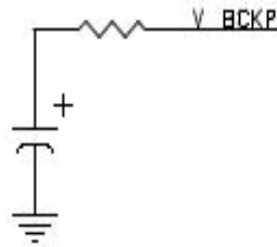
Figure 4: Example Voltage Backup connection
