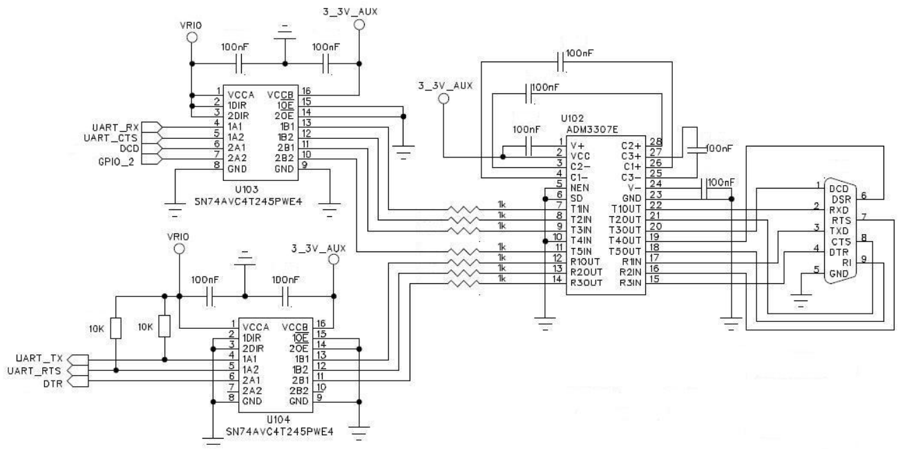
Figure 8: Level-shifter connection to RS232
