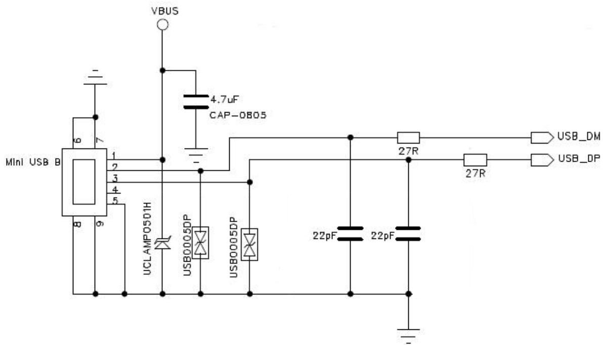
Figure 9: Example of USB implementation
