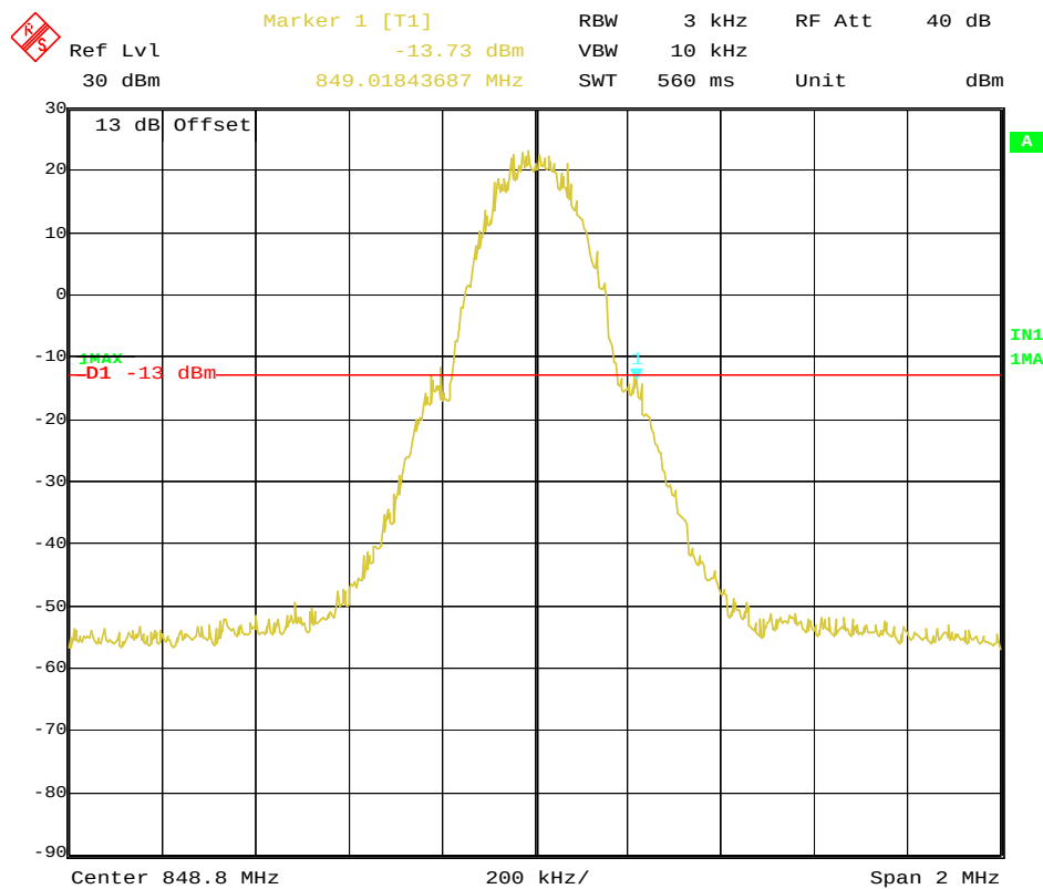
GSM850 Channel 251 Right band edge
