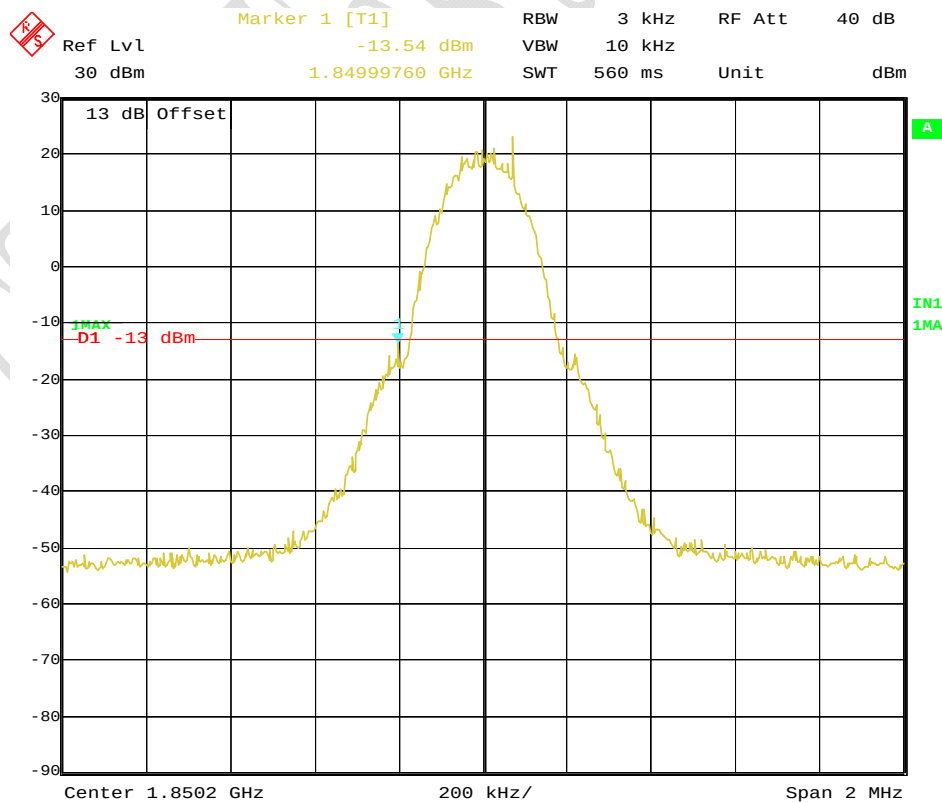
GSM1900 Channel 512 Left band edge
