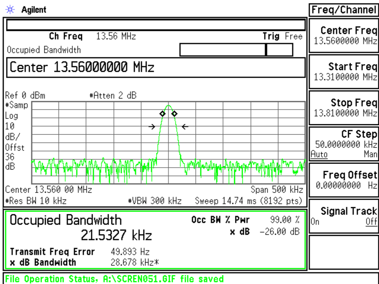
Figure 2: Occupied Bandwidth
