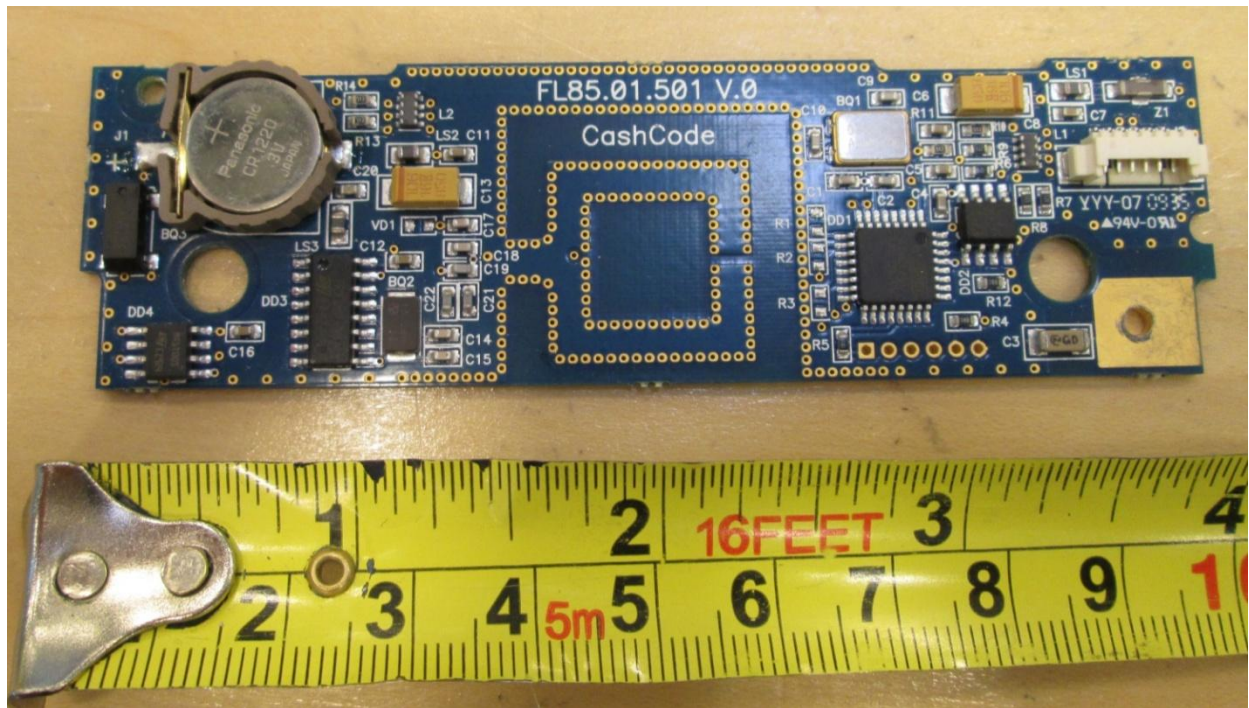
Part #1. RFID board, side 1
