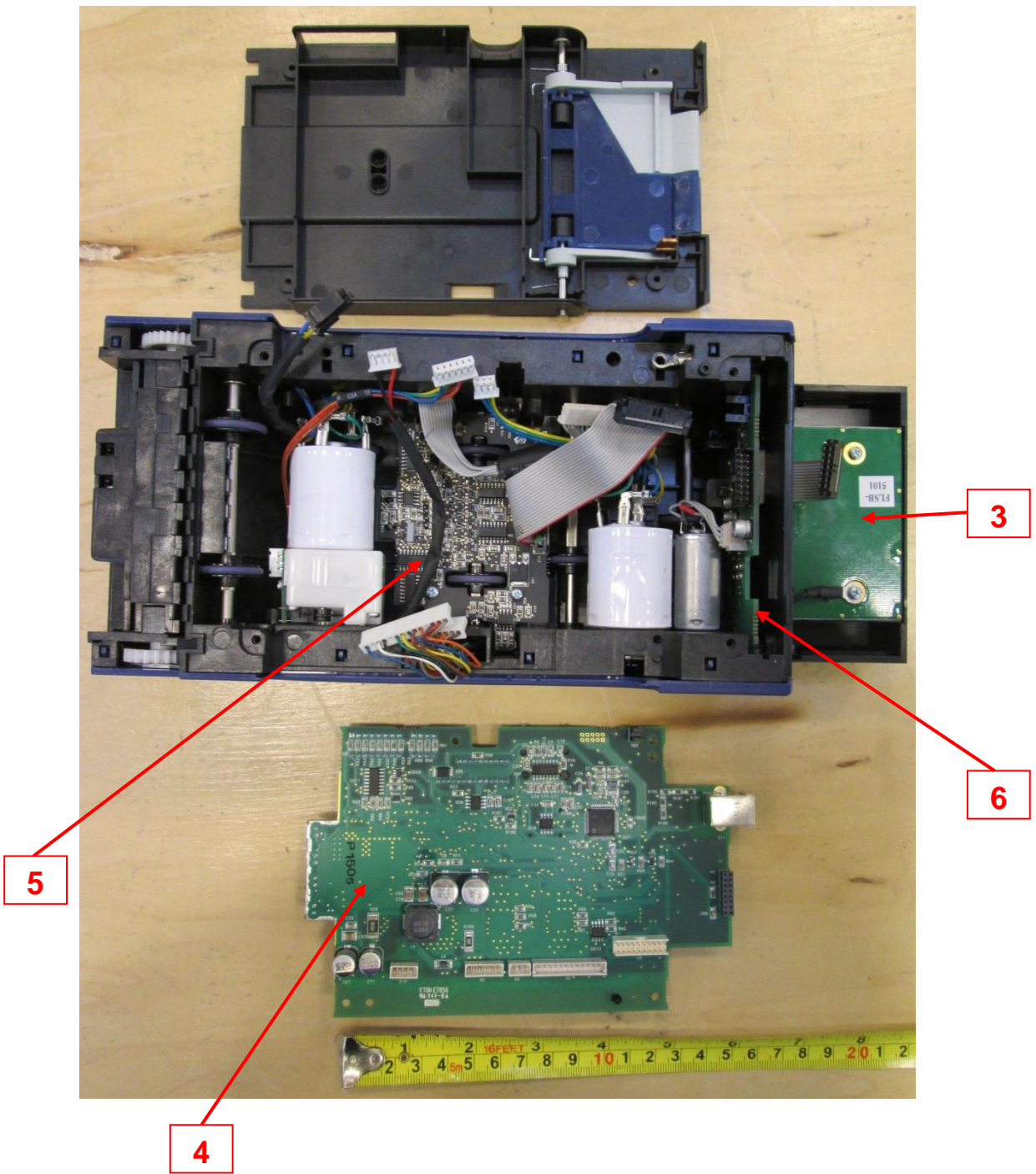
Part #2. Internal view, with board removed
