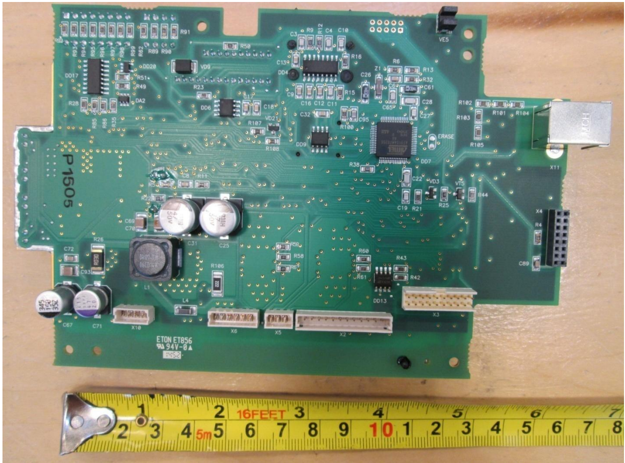
Part #4. Side 1
