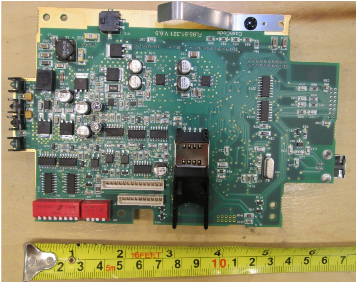
Part #4. Side 2
