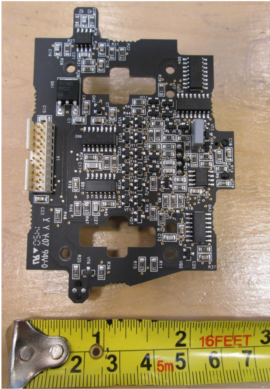
Part #5. Side 1
