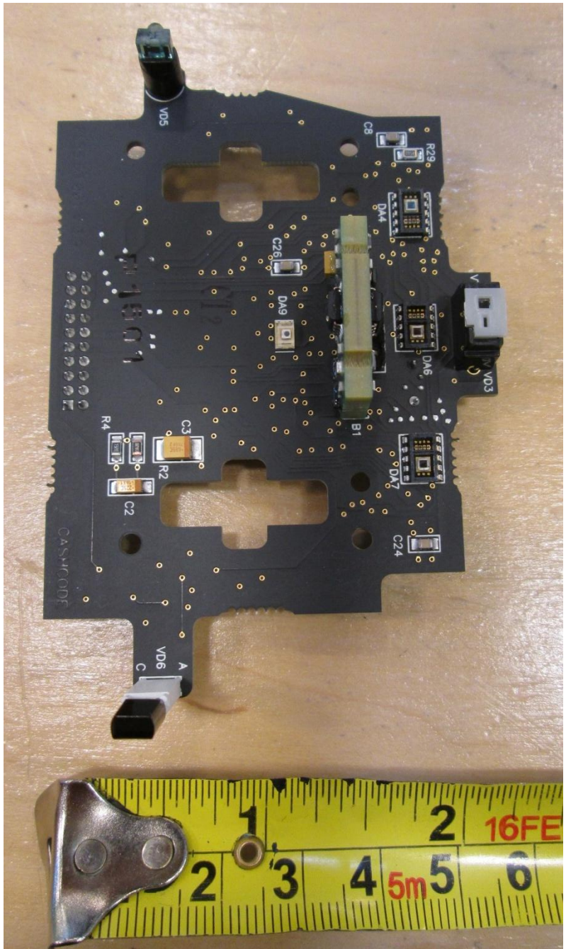
Part #5. Side 2
