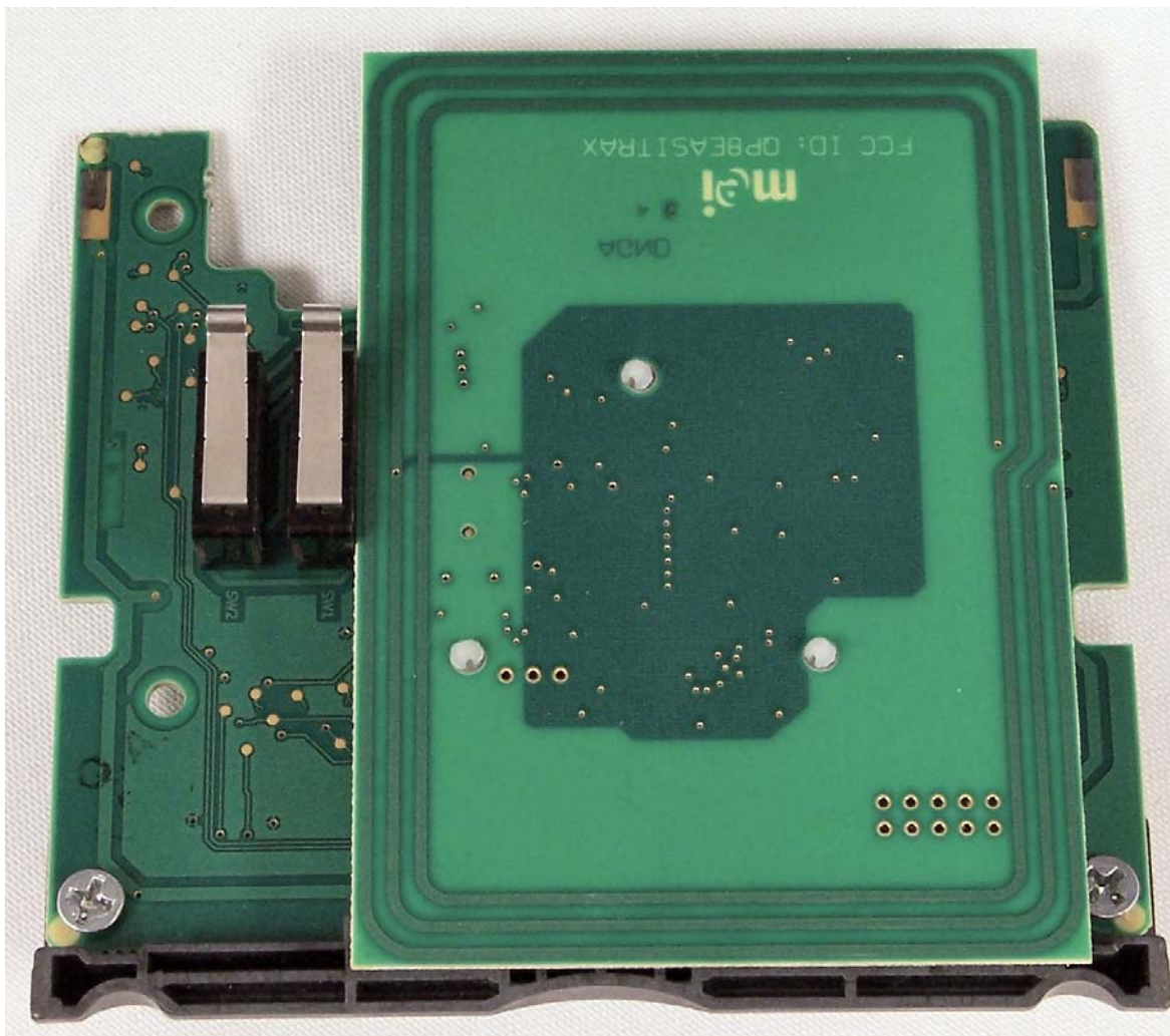
Radio Card / Antenna Side (Mounted on Parent Board)
