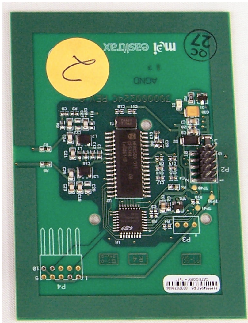
Radio Card
