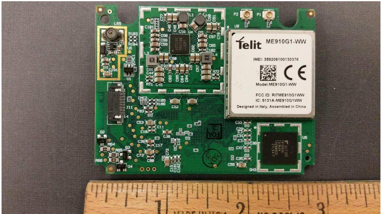
PIC 1 A – 111556844C, ALIO Note PCMA board, Front
