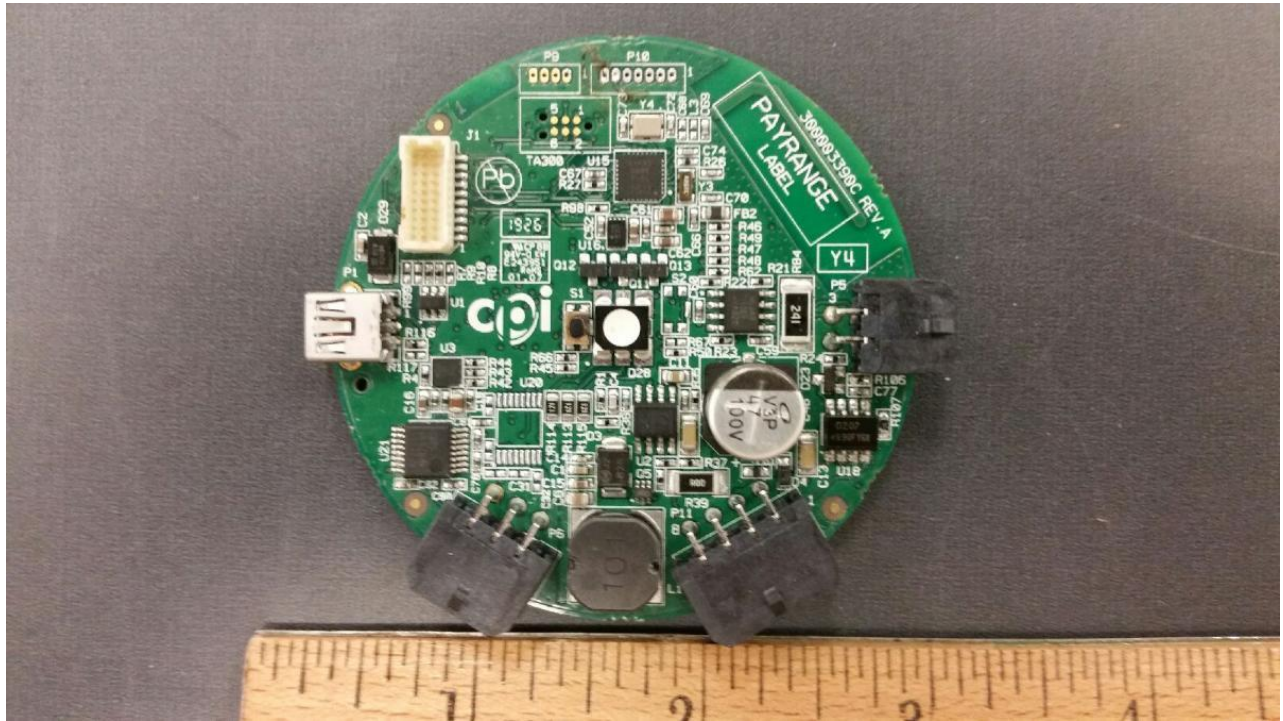
PIC 3 A – 111550788C, RXIA (BLE) board, Front
