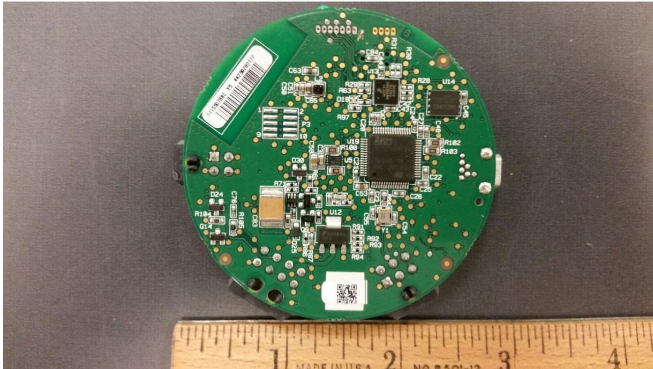
PIC 3 B – 111550788C, RXIA (BLE) board, Back
