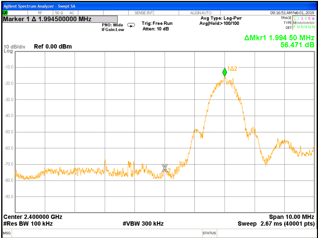
Figure 1: Lower Bandedge
