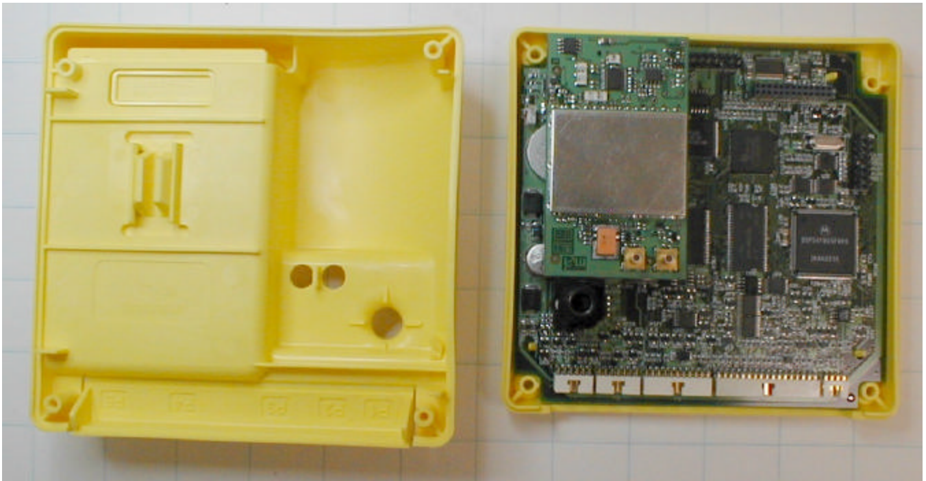
Cover Removed
