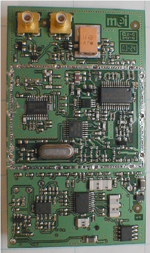
Radio Module Top View (Shield Removed)
