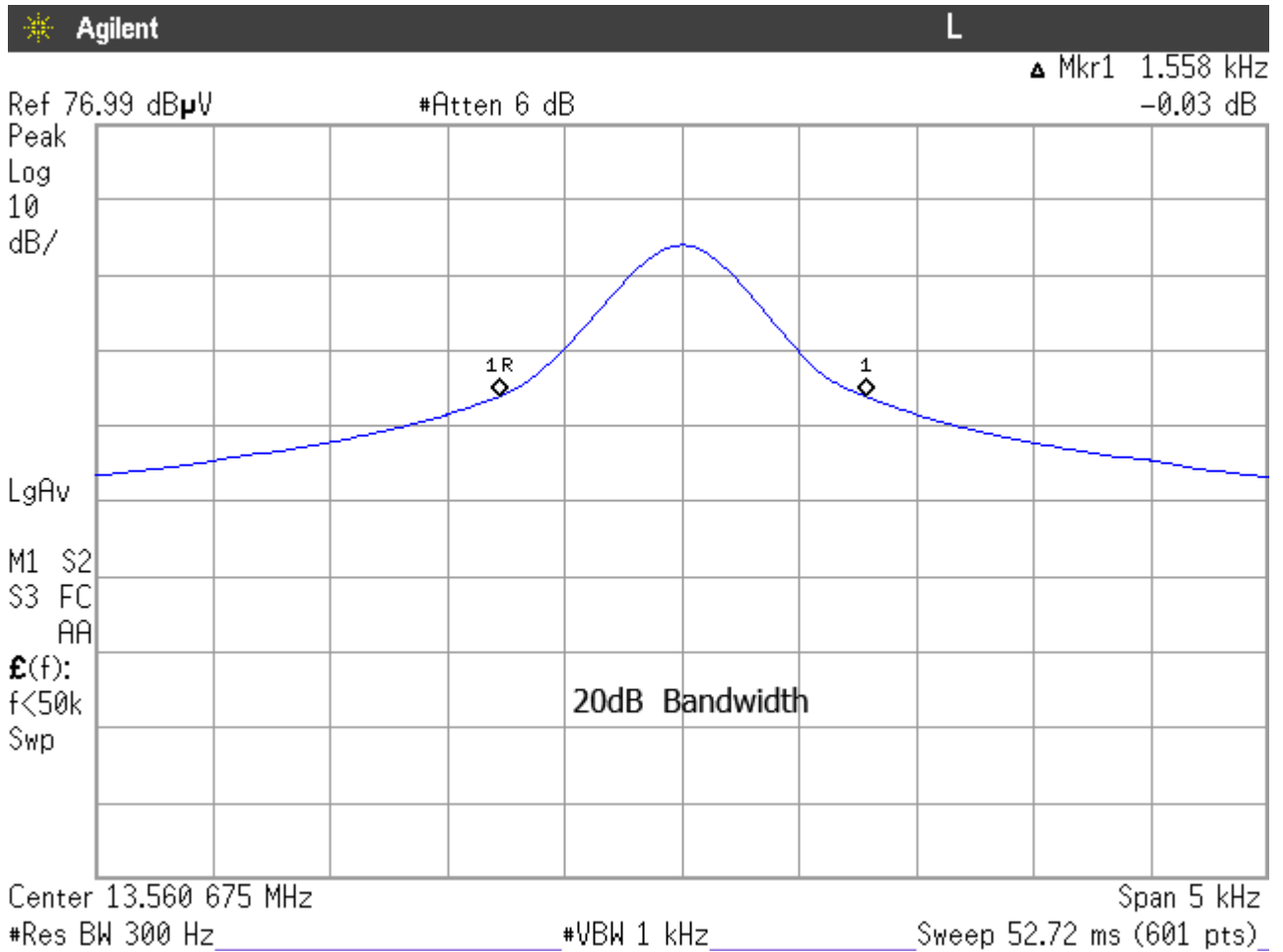
Figure 2: Occupied Bandwidth
