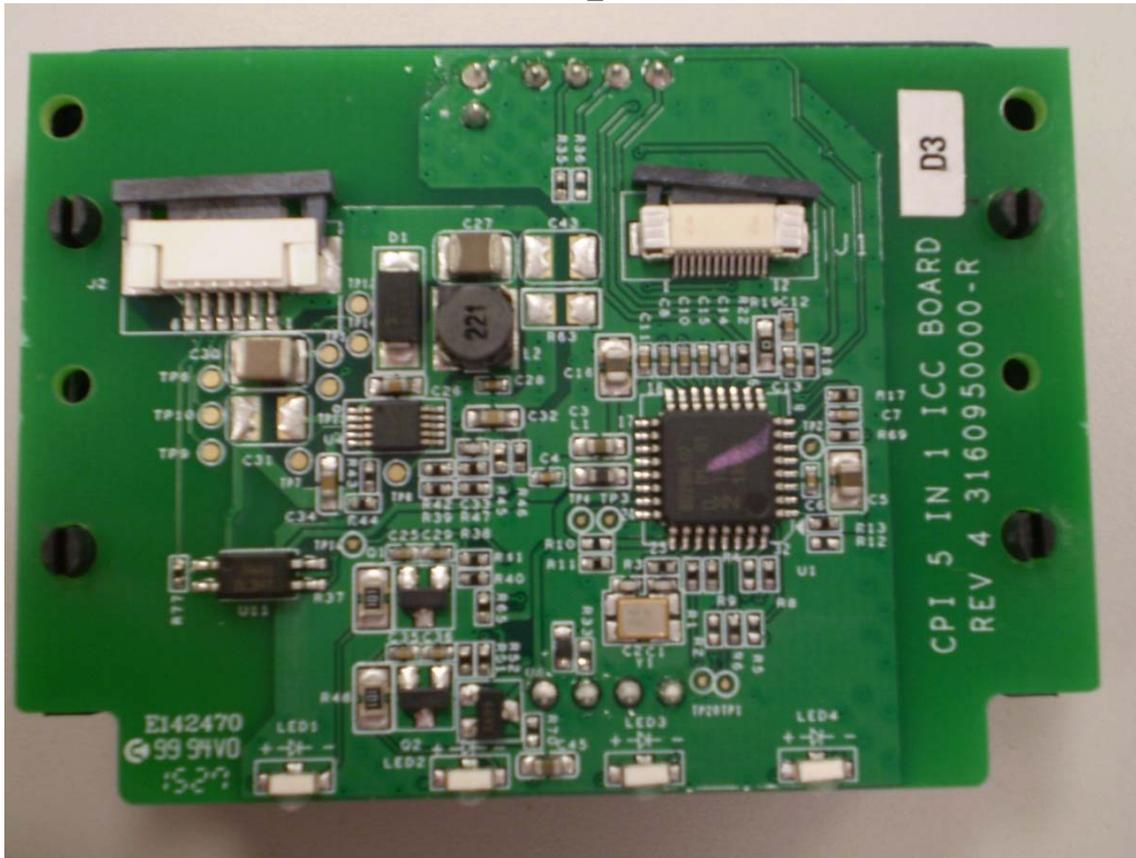
ICC PCB_Back
