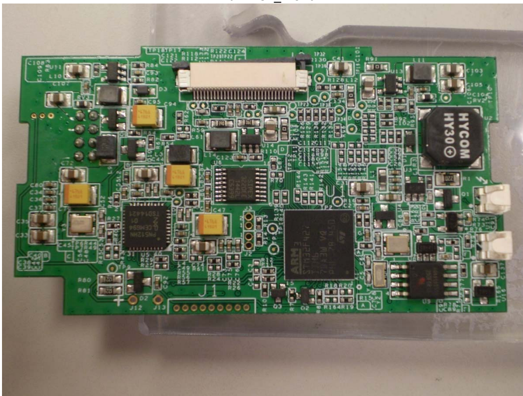
Main PCB_Front
