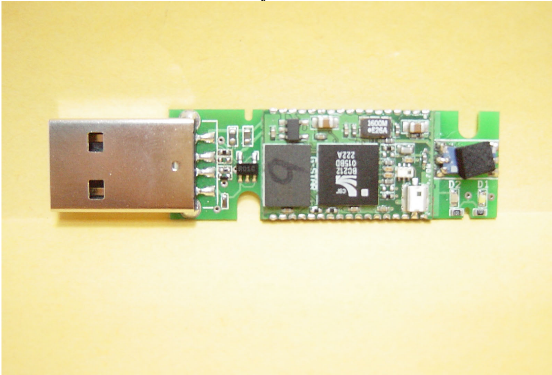
Internal of EUT - Front
