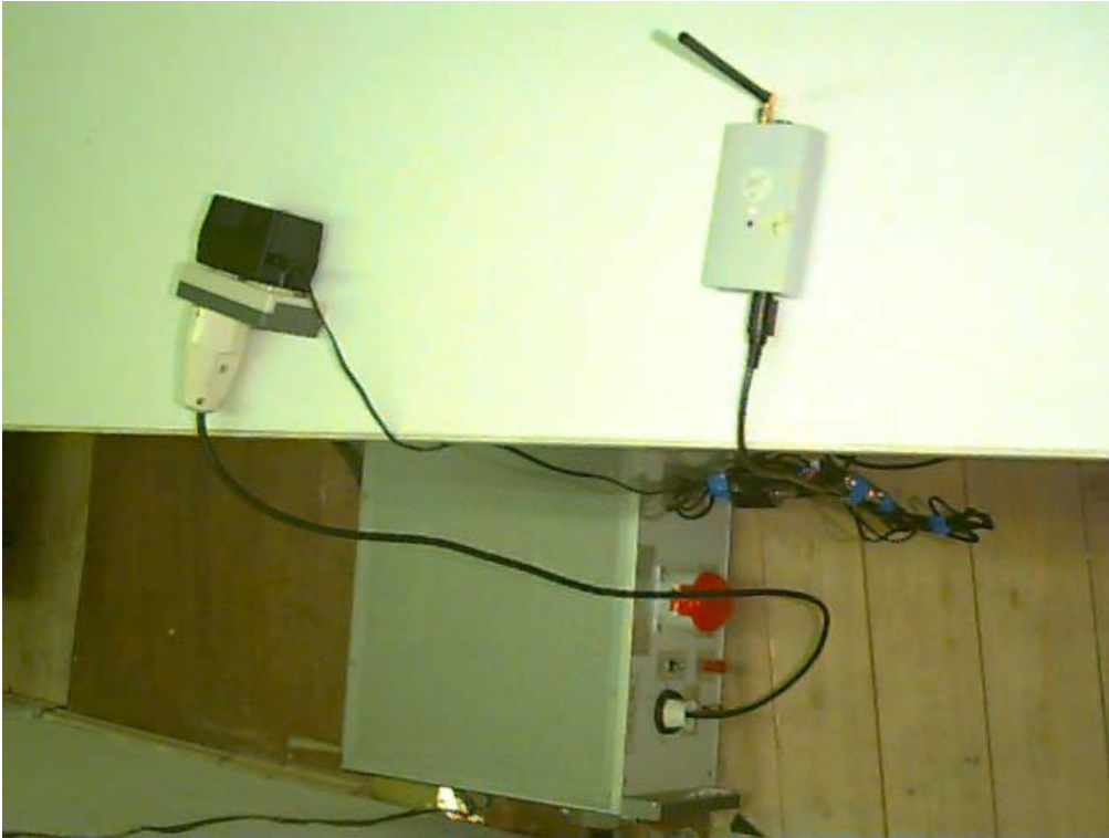
EUT supplied via RS485 from FRIWO FW1199
