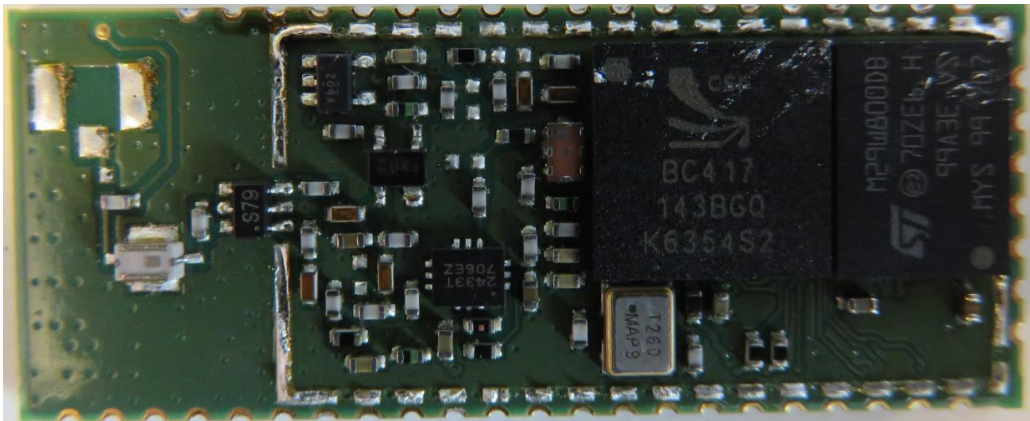
Figure 2: WT41u-N Internal View
