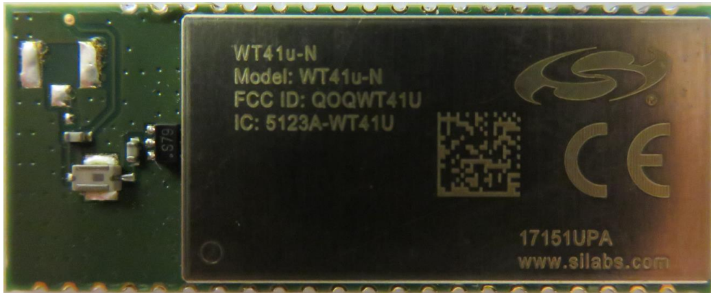
Figure 1: WT41u-N Top View
