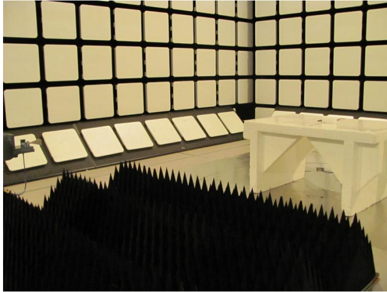
Photograph 3. Radiated emissions 18-26.5 GHz
