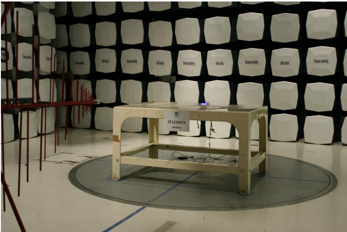
Radiated Emissions Test Setup (below 1GHz)
