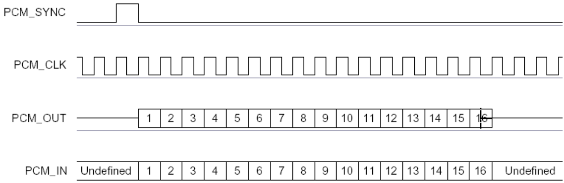
Figure 16: Short Frame Sync (Shown with 16-bit Sample)
