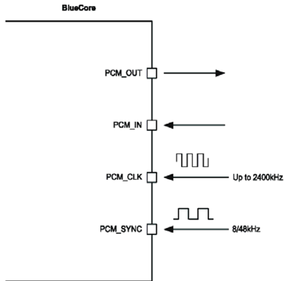
Figure 14: WT21 as a PCM Interface Slave
