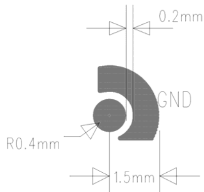
Figure 33: Dimensions of the RFTP
