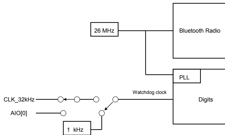
Figure 4: Clock Architecture
