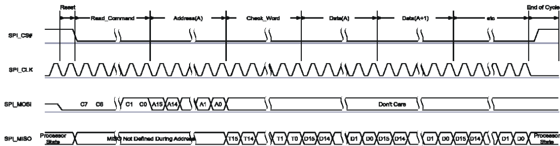
Figure 6: SPI Read Operation
