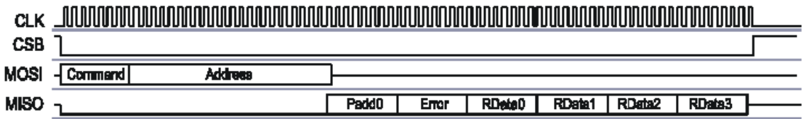
Figure 12: CSPI Burst Read Cycle
