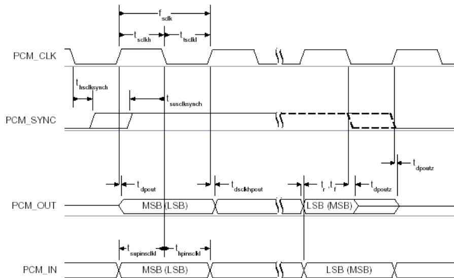
Figure 23: PCM Slave Timing Long Frame Sync
