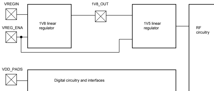
Figure 28: Voltage Regulator Configuration
