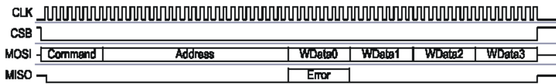
Figure 11: CSPI Burst Write Cycle
