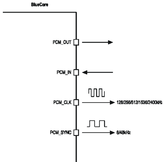
Figure 13: WT21 as a PCM Interface Master
