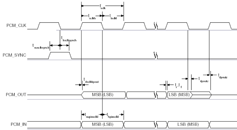
Figure 24: PCM Slave Timing Short Frame Sync
