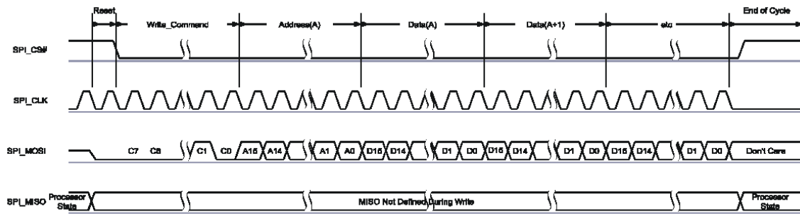
Figure 5: SPI Write Operation
