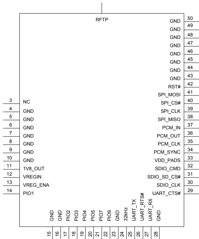
Figure 1: WT21 pin out
