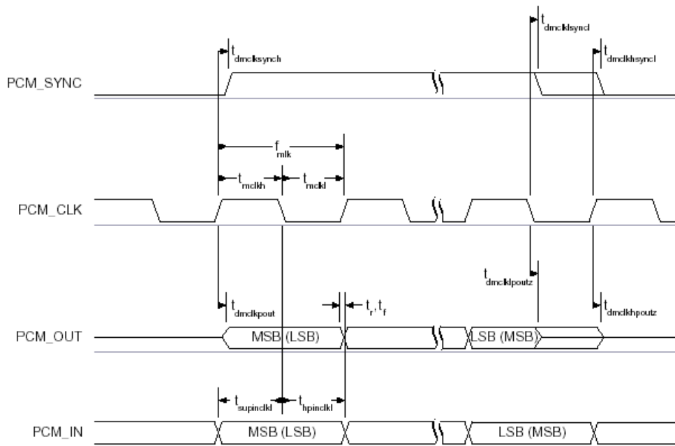
Figure 21: PCM Master Timing Long Frame Sync
