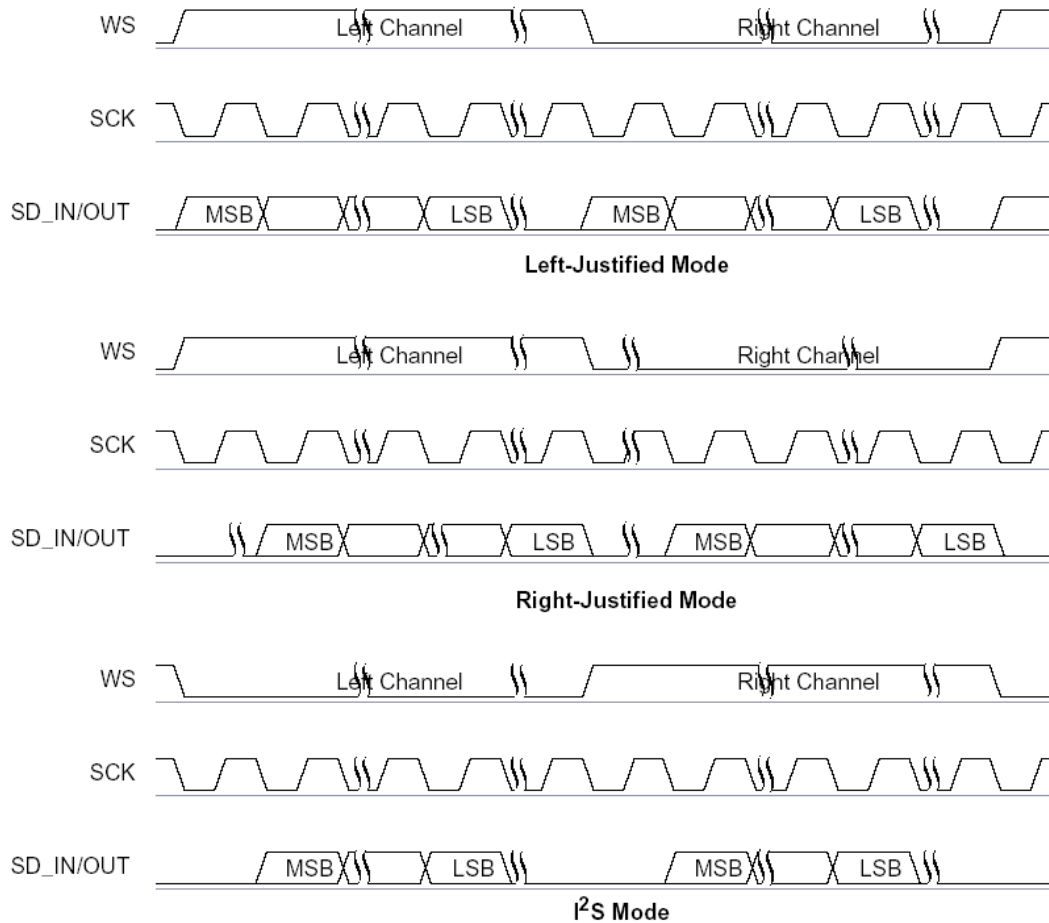
Figure 25: Digital Audio Interface Modes
