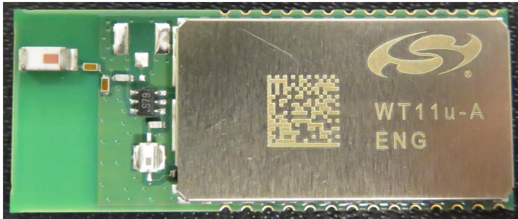
Figure 2: WT11u-A, external, top view
