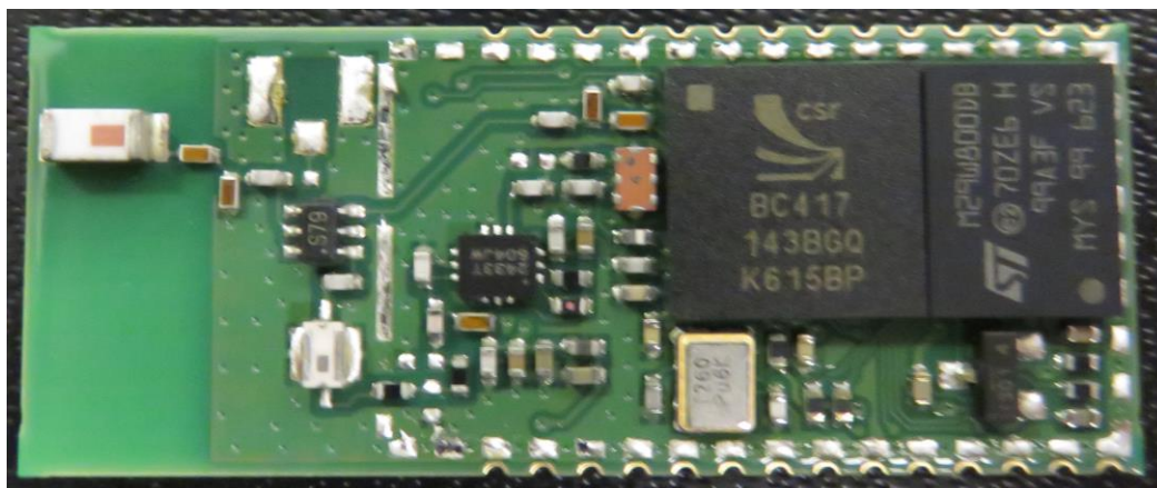
Figure 3: WT11u-A, internal, top view
