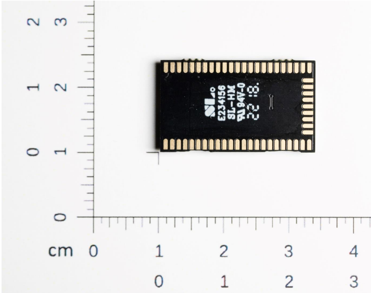
Figure 2: Bottom (rear) view of "A" variant
