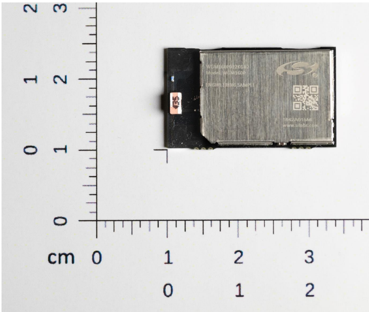
Figure 1: Top (front) external view of “A” variant with integral antenna
