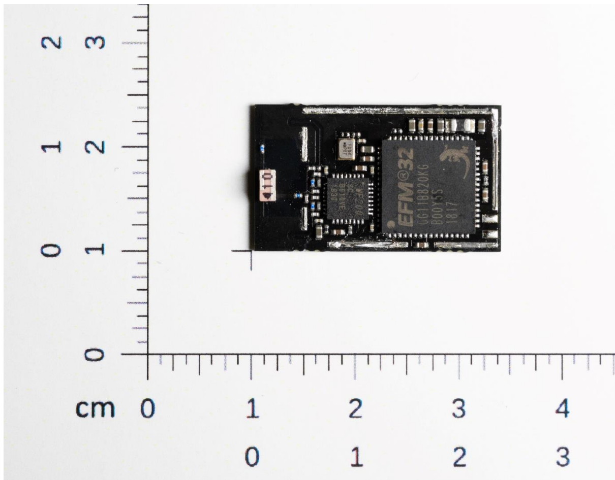
Figure 1: Top (front) internal view of "A" variant with integral antenna
