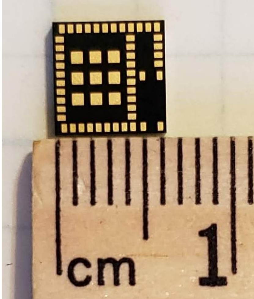
Figure 2: Bottom (rear) view of WFM200SA and WFM200SN
