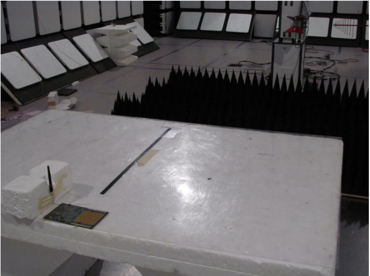
Radiated emissions test setup model WF121-E
