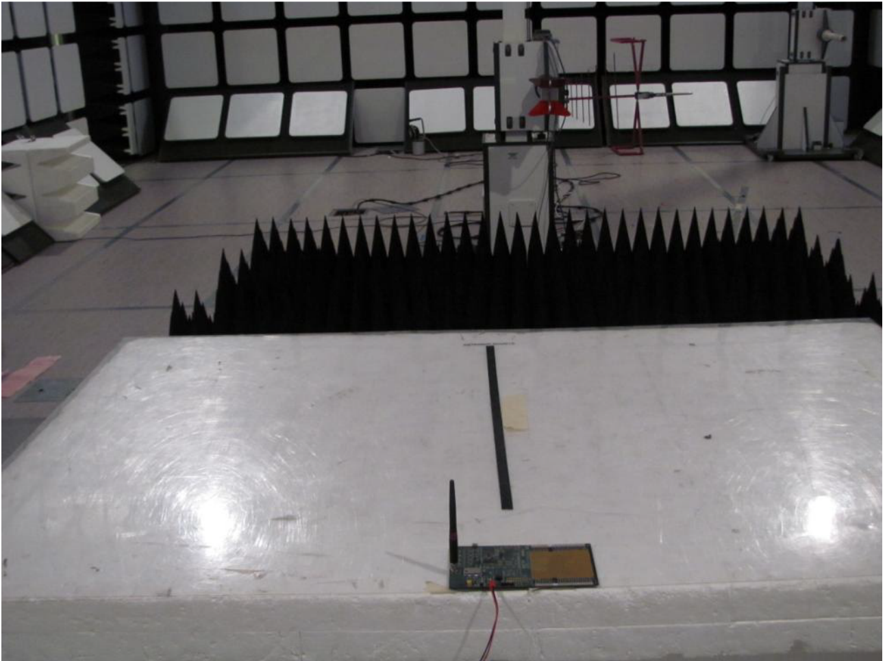
Radiated emission test setup model WF121-N
