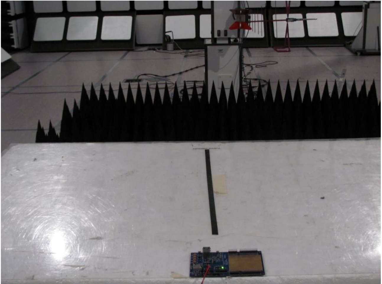
Radiated emissions test setup model WF121-A
