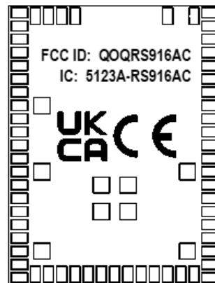
SILK SCREEN (BOTTOM)
