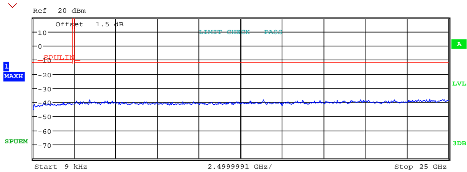
Out of Band Emissions – 2442 MHz
