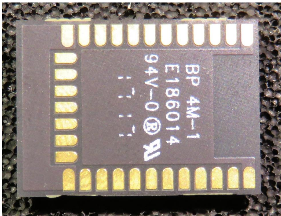
Figure 2: MGM13PxxxxE/A, external, bottom view
