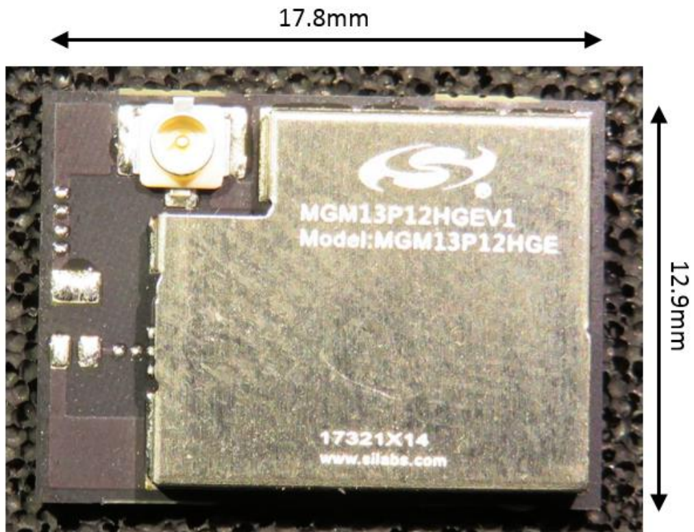
Figure 1: MGM13PxxxxE, external, top view
