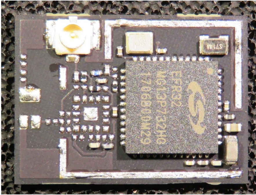
Figure 5: MGM13PxxxE, internal, top view
