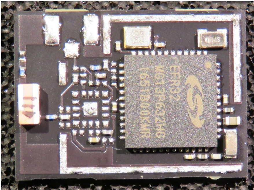
Figure 4: MGM13PxxxxA, internal, top view
