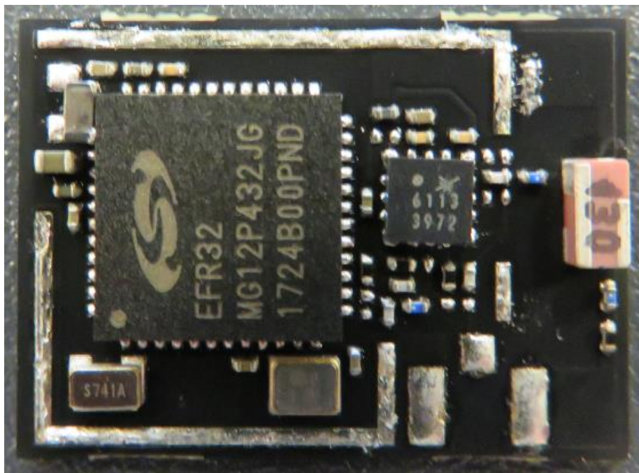
Figure 2: MGM12P32GA Internal, Top View
