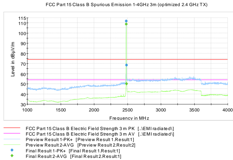
Figure 28: High channel 1 GHz – 4 GHz (E)
