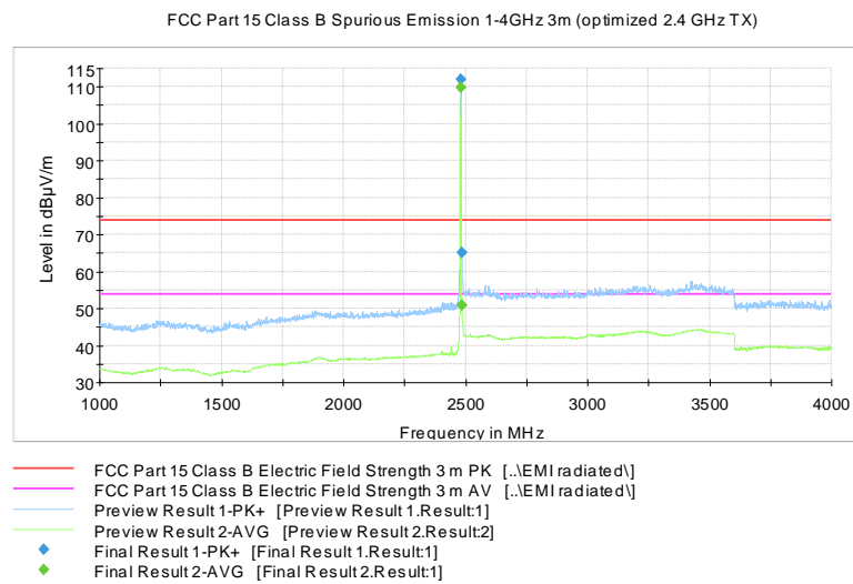
Figure 14: High channel 1 GHz – 4 GHz (A)
