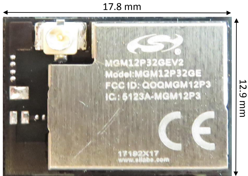
Figure 1: MGM12P32GE, external, top view
