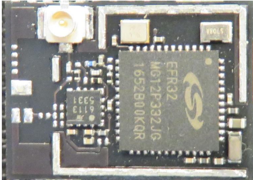
Figure 3: MGM12P32GE, internal, top view
