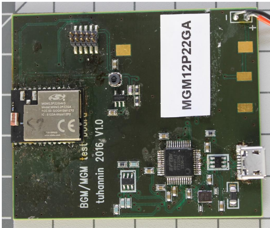
Photograph 1. EUT
