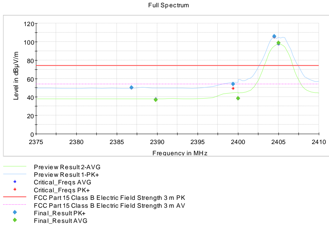
Figure 14: Radiated Band Edge measurement graph, Channel 11 low
