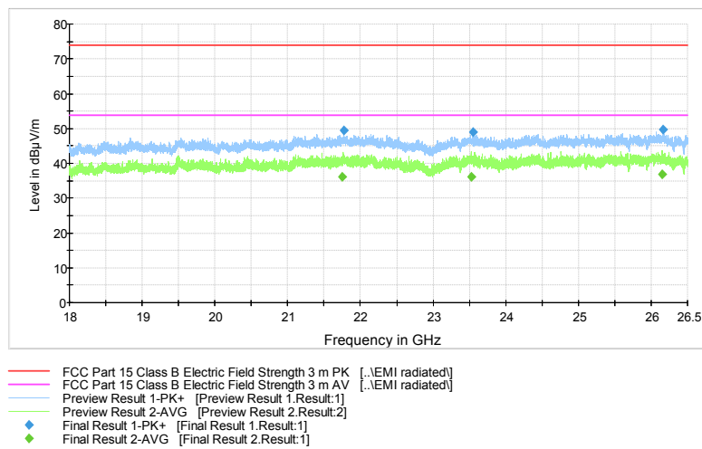
Figure 17: High channel 18 GHz – 26.5 GHz
