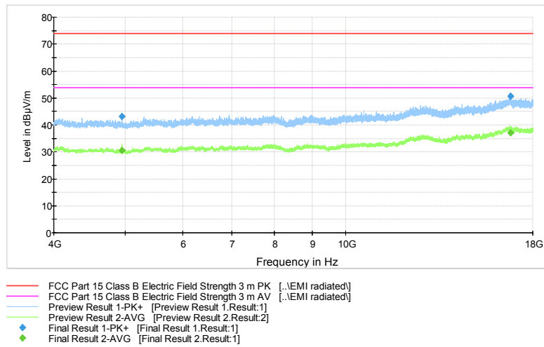
Figure 16: High channel 4 GHz – 18 GHz
