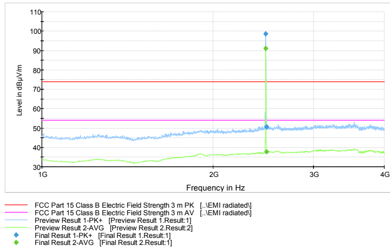
Figure 15: High channel 1 GHz – 4 GHz
