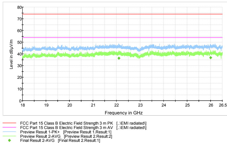
Figure 32: High channel 18 GHz – 26.5 GHz
