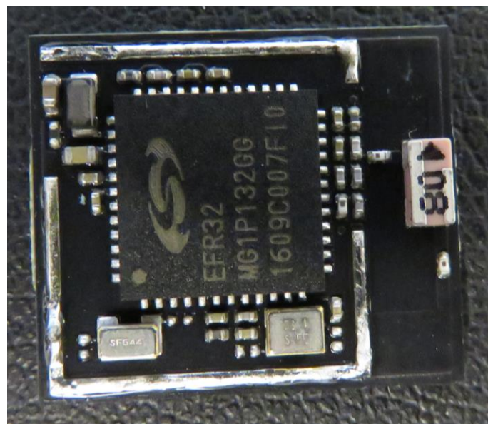
Figure 2: MGM111A internal, top view
