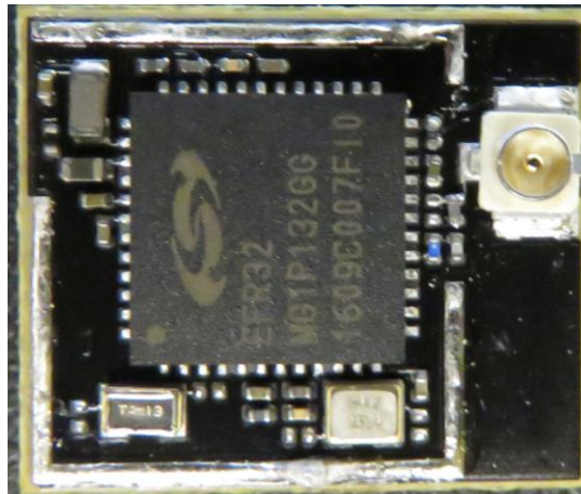
Figure 4: MGM111E internal, top view
