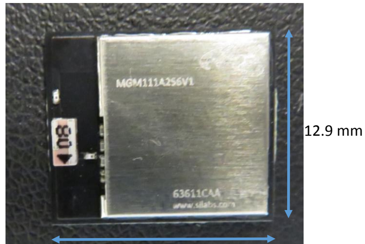
Figure 1: MGM111A external, top view
