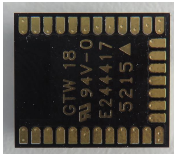
Figure 5: MGM111A and MGM111E bottom view
