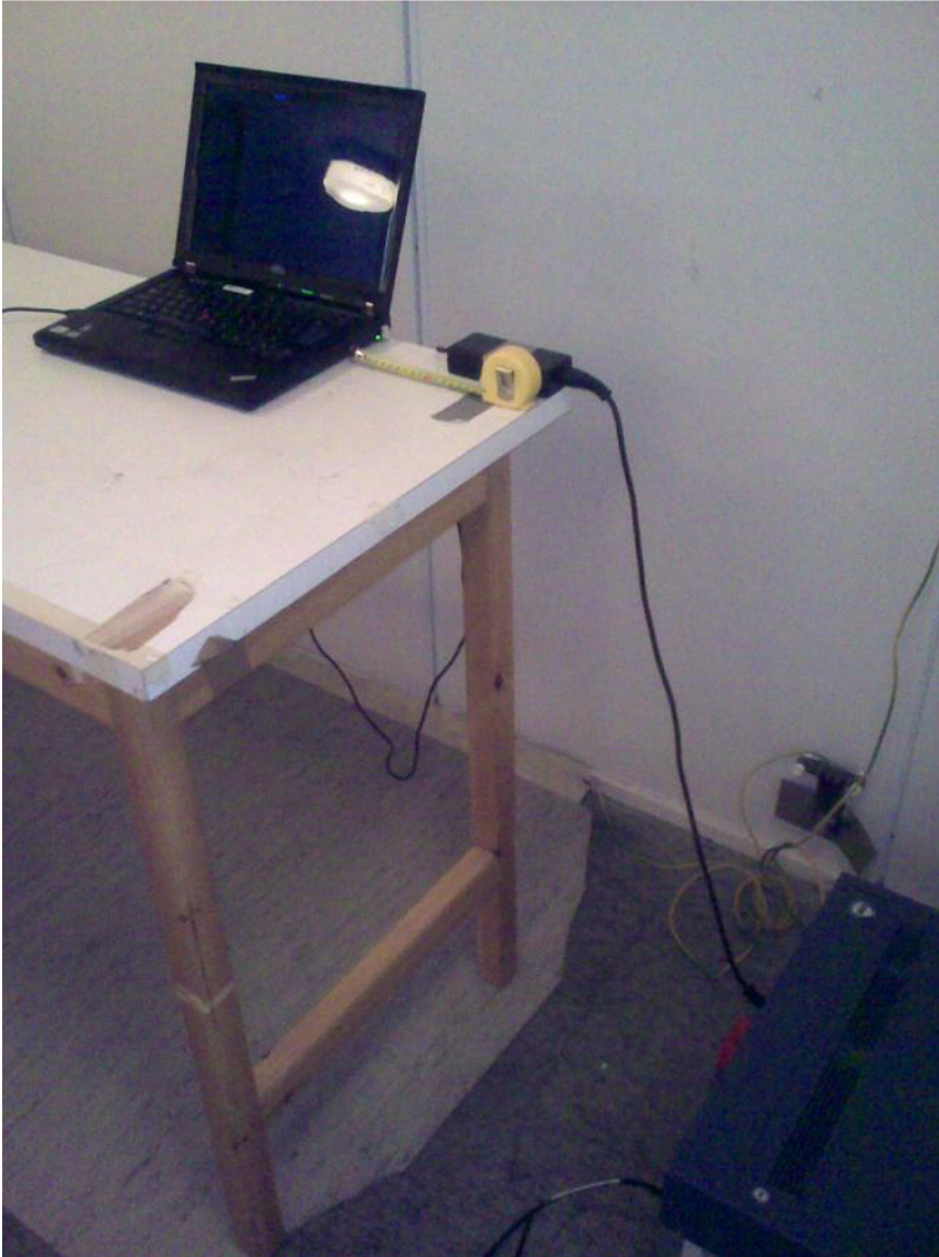
Conducted emissions test setup.
