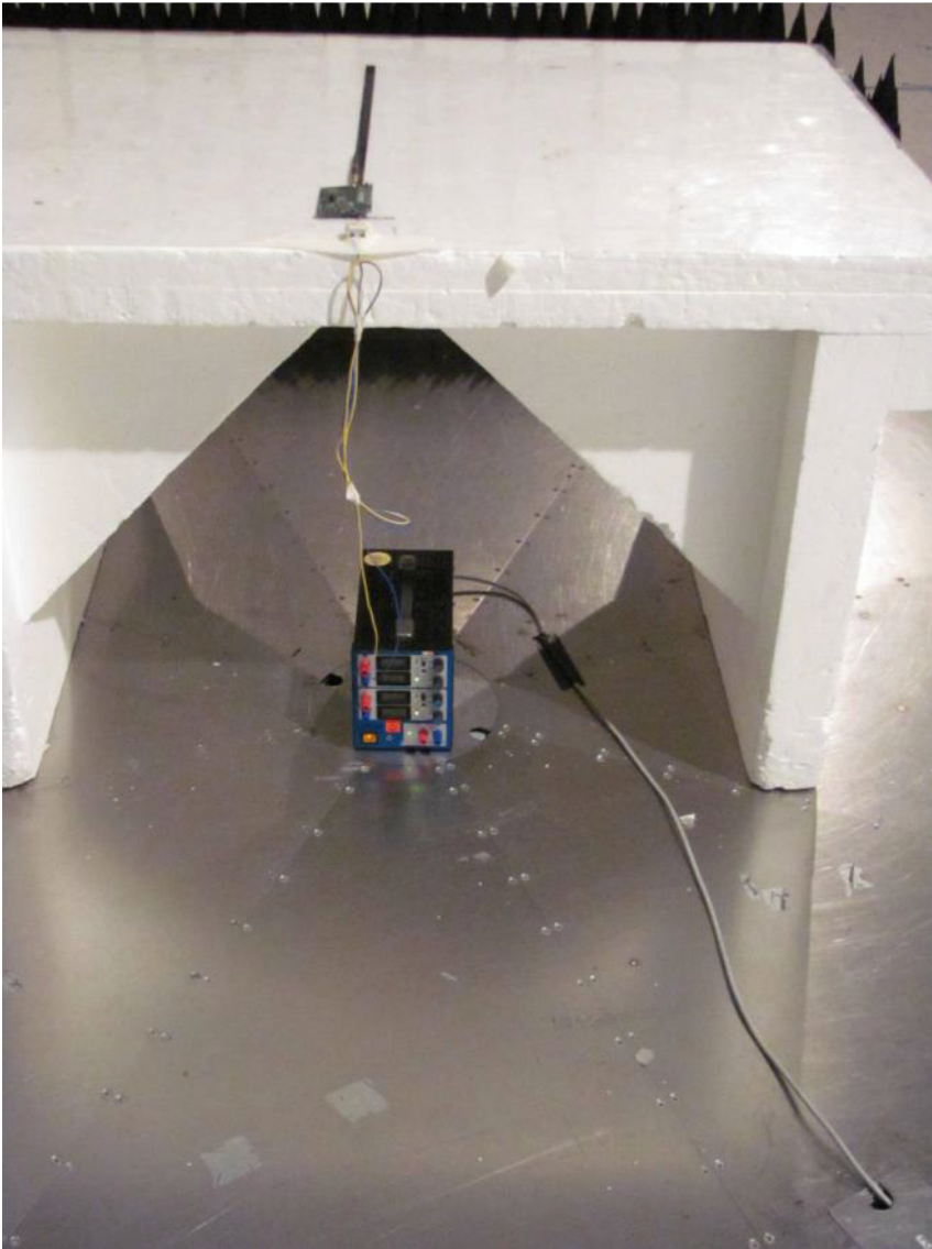
Radiated emission test setup.
