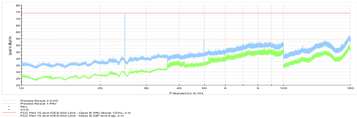
Figure 8.4-6: Radiated spurious emissions 1 to 18 GHz with antenna 1, High channel
