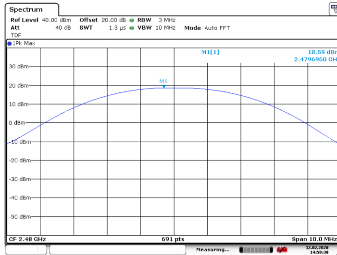
Figure 8.3-6: Conducted output power, high channel
