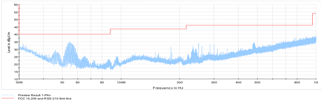
Figure 8.4-14: Radiated spurious emissions 30 MHz to 1 GHz with antenna 3, mid channel
