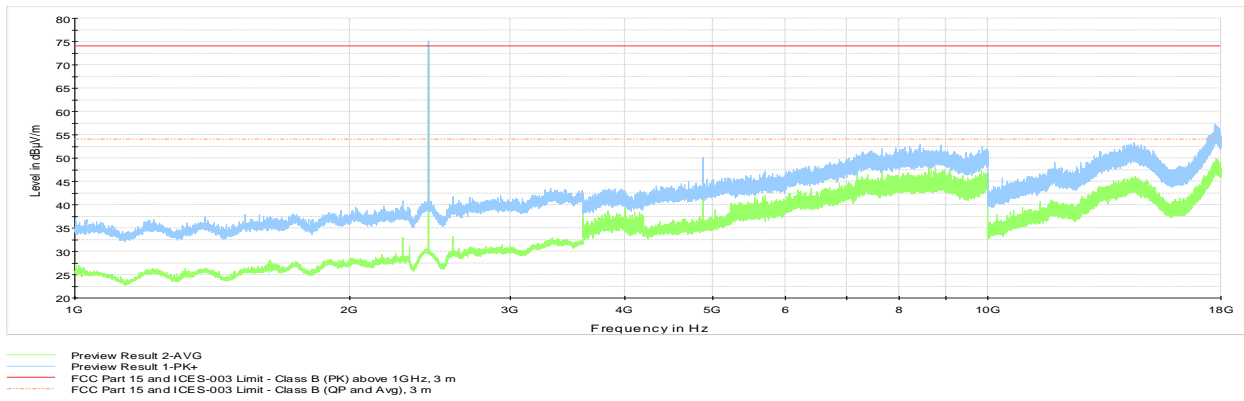
Figure 8.4-17: Radiated spurious emissions 1 to 18 GHz with antenna 3, mid channel
