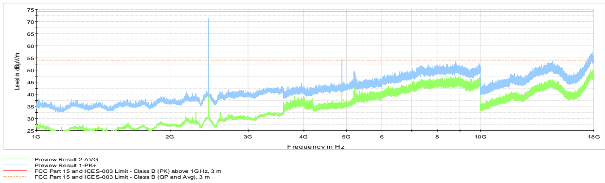
Figure 8.4-5: Radiated spurious emissions 1 to 18 GHz with antenna 1, mid channel
