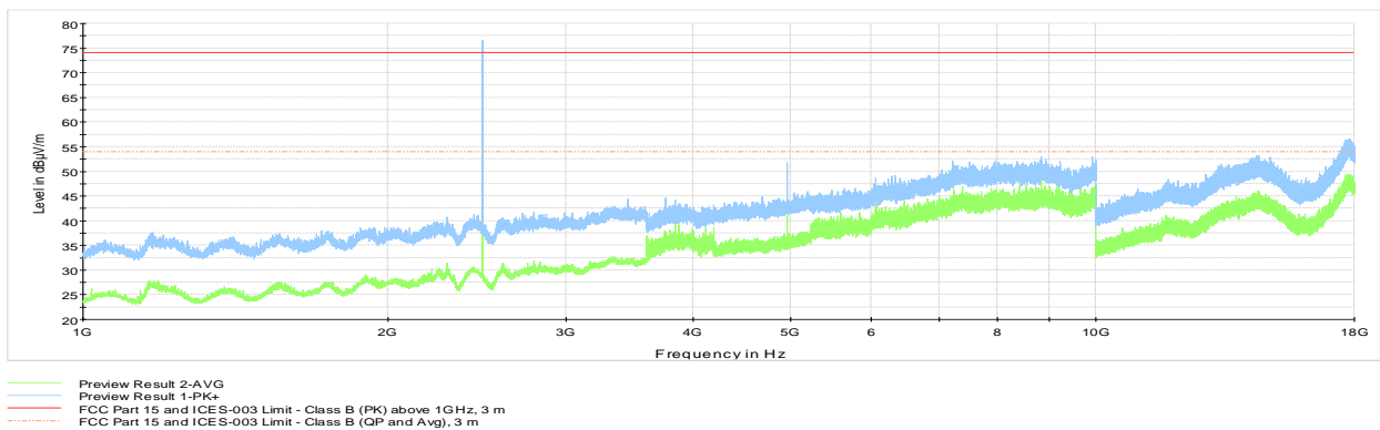
Figure 8.4-12: Radiated spurious emissions 1 to 18 GHz with antenna 2, High channel
