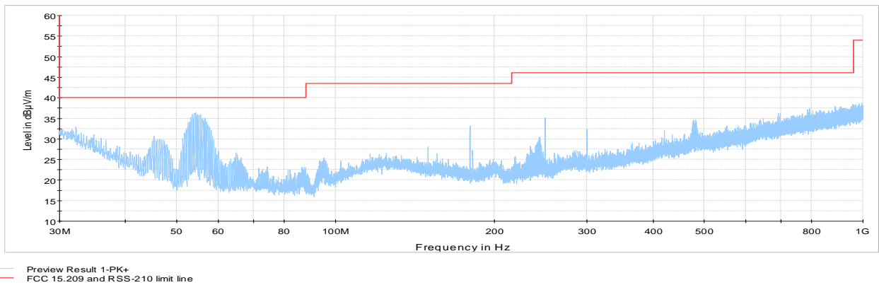
Figure 8.4-2: Radiated spurious emissions 30 MHz to 1 GHz with antenna 1, mid channel
