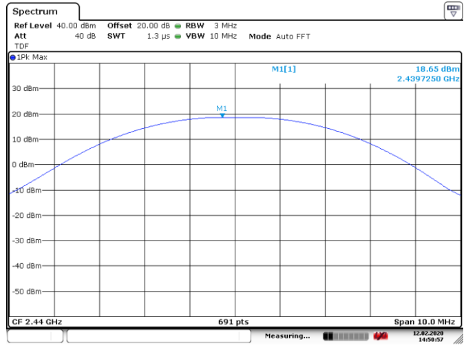
Figure 8.3-5 Conducted output power, mid channel
