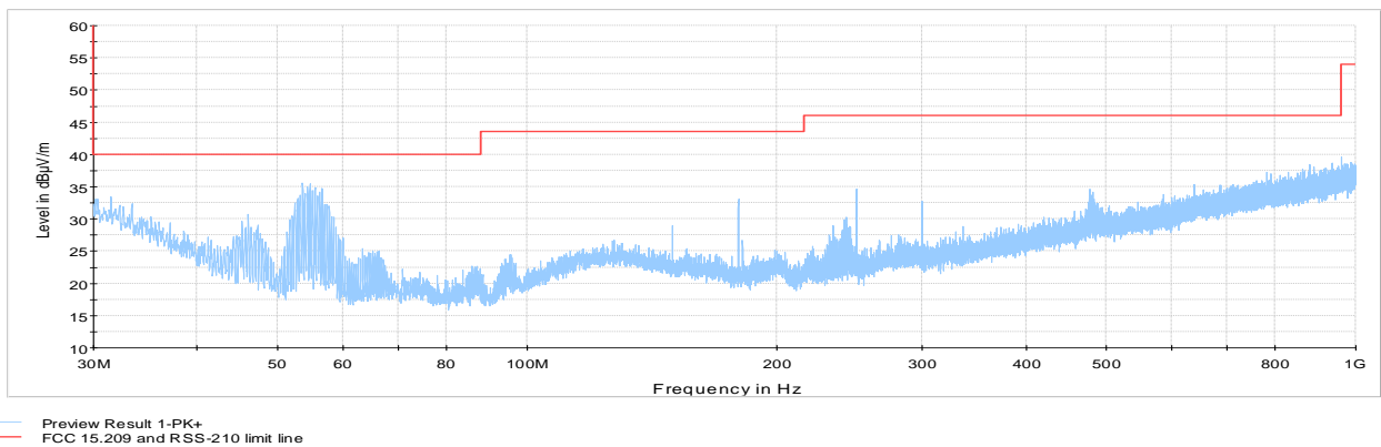
Figure 8.4-3: Radiated spurious emissions 30 MHz to 1 GHz with antenna 1, High channel
