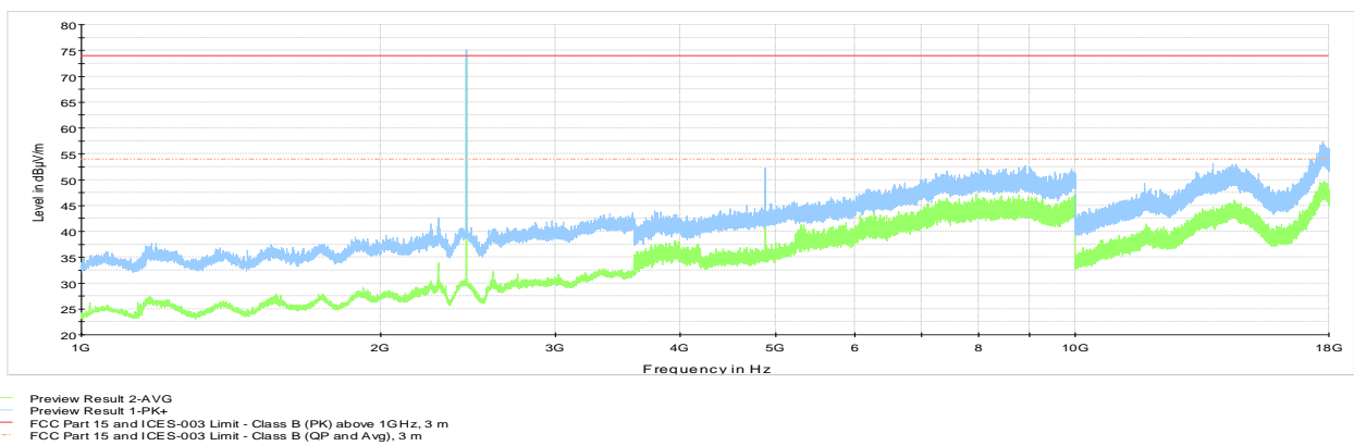
Figure 8.4-11: Radiated spurious emissions 1 to 18 GHz with antenna 2, mid channel
