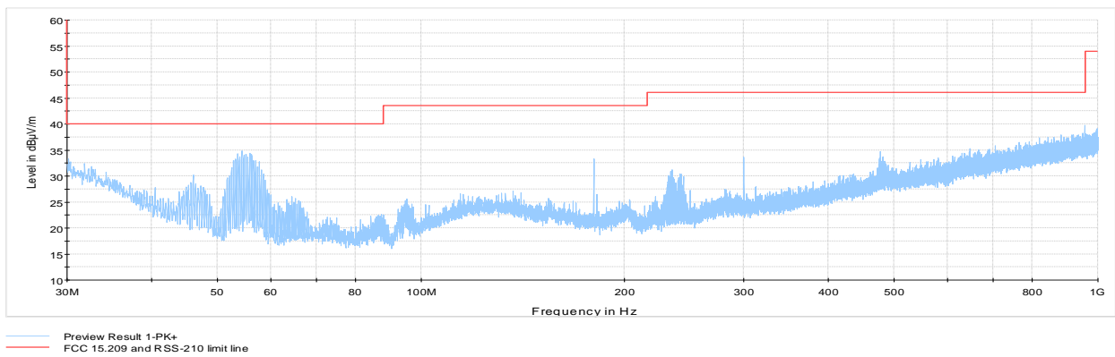
Figure 8.4-8: Radiated spurious emissions 30 MHz to 1 GHz with antenna 2, mid channel
