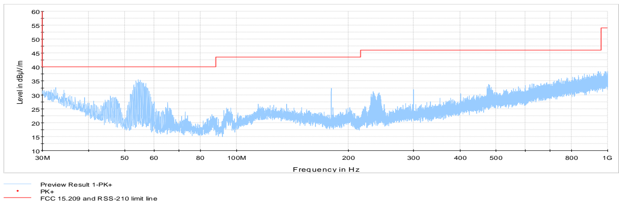
Figure 8.4-9: Radiated spurious emissions 30 MHz to 1 GHz with antenna 2, High channel
