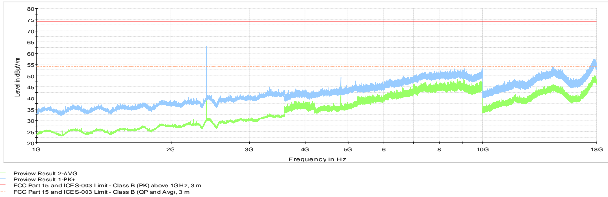
Figure 8.4-22: Radiated spurious emissions 1 to 18 GHz with antenna 4, Low channel
