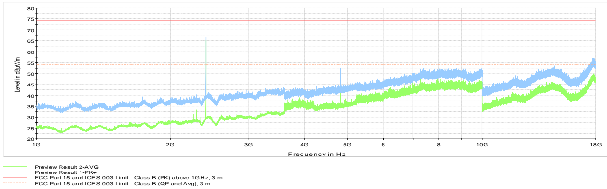
Figure 8.4-16: Radiated spurious emissions 1 to 18 GHz with antenna 3, Low channel
