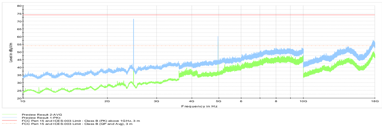
Figure 8.4-24: Radiated spurious emissions 1 to 18 GHz with antenna 4, High channel
