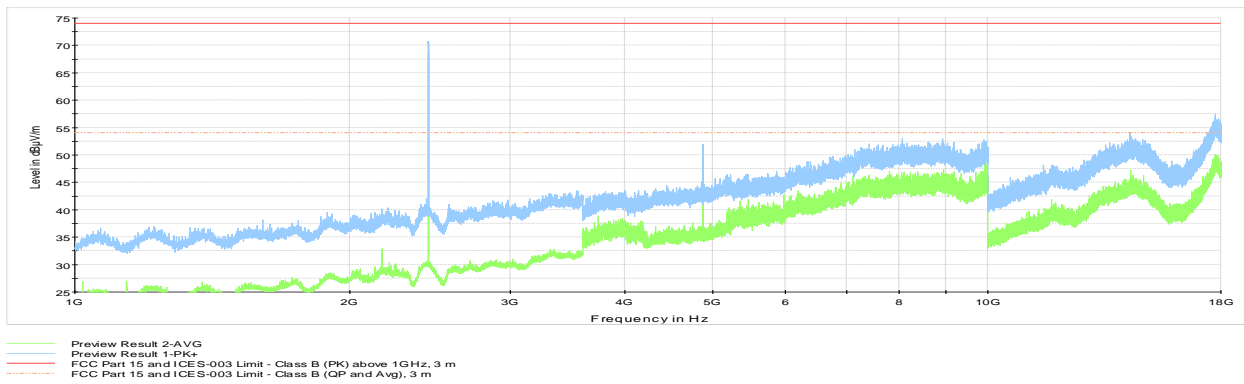
Figure 8.4-23: Radiated spurious emissions 1 to 18 GHz with antenna 4, mid channel
