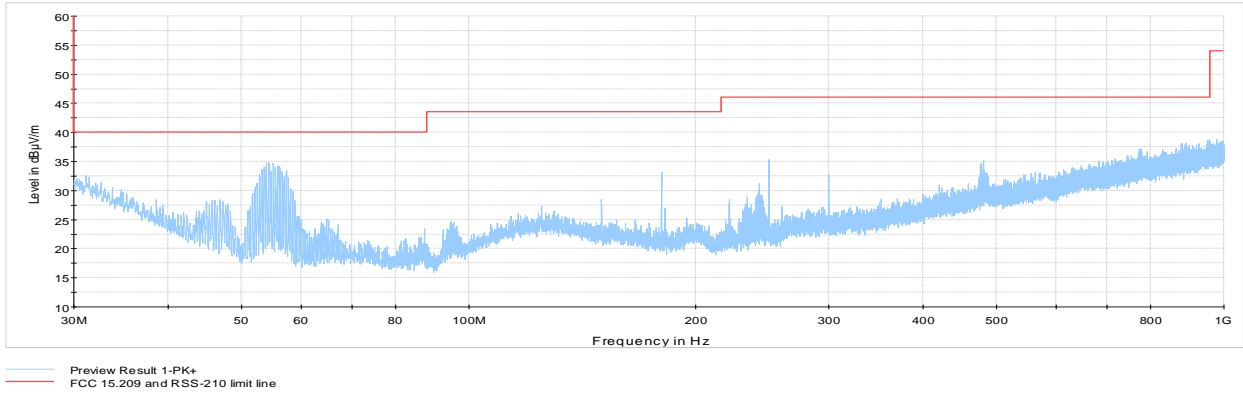
Figure 8.4-1: Radiated spurious emissions 30 MHz to 1 GHz with antenna 1, Low channel
