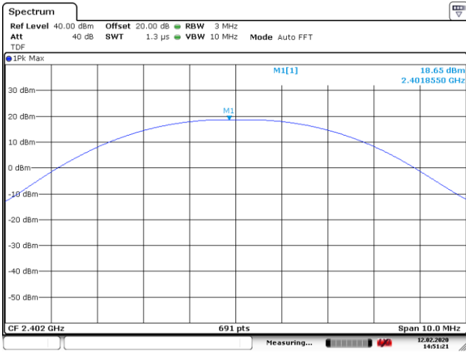
Figure 8.3-4: Conducted output power, low channel
