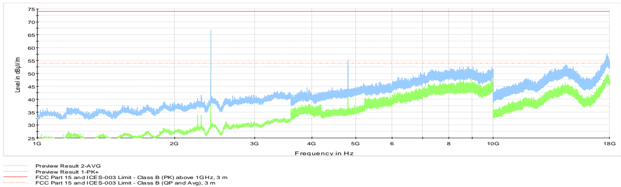
Figure 8.4-10: Radiated spurious emissions 1 to 18 GHz with antenna 2, Low channel
