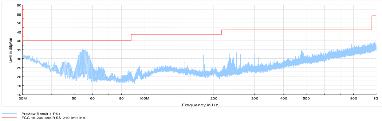
Figure 8.4-13: Radiated spurious emissions 30 MHz to 1 GHz with antenna 3, Low channel
