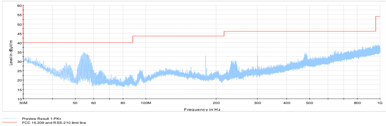
Figure 8.4-7: Radiated spurious emissions 30 MHz to 1 GHz with antenna 2, Low channel
