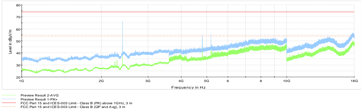
Figure 8.4-4: Radiated spurious emissions 1 to 18 GHz with antenna 1, Low channel
