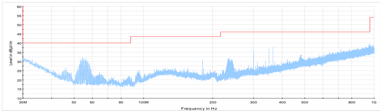
— Preview Result 1-PK+ — FCC 15.209 and RSS-210 limit line
