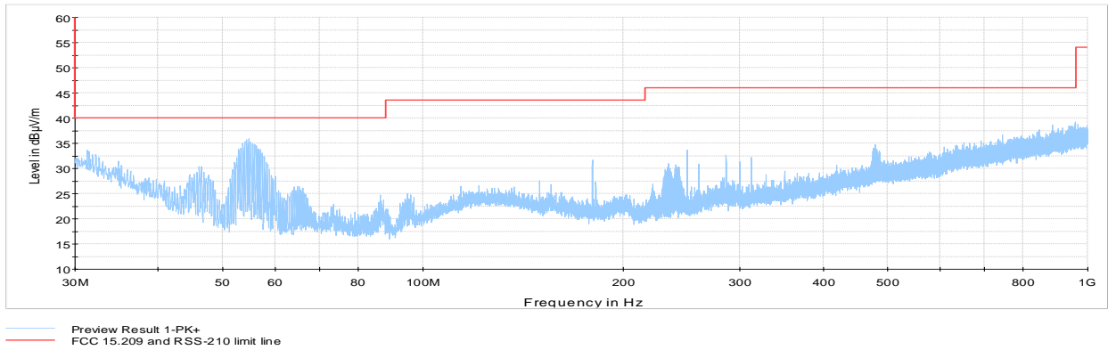
Figure 8.4-15: Radiated spurious emissions 30 MHz to 1 GHz with antenna 3, High channel
