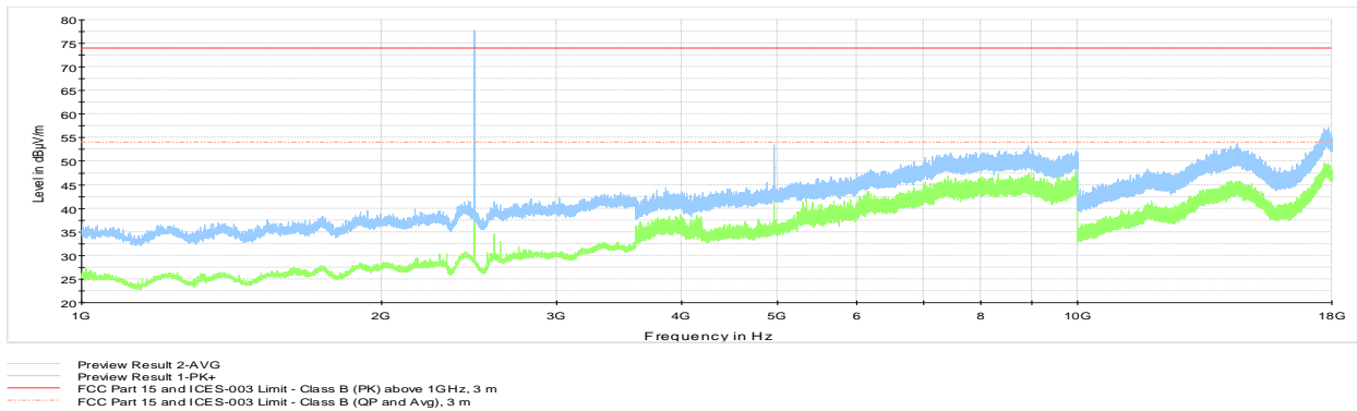
Figure 8.4-18: Radiated spurious emissions 1 to 18 GHz with antenna 3, High channel
