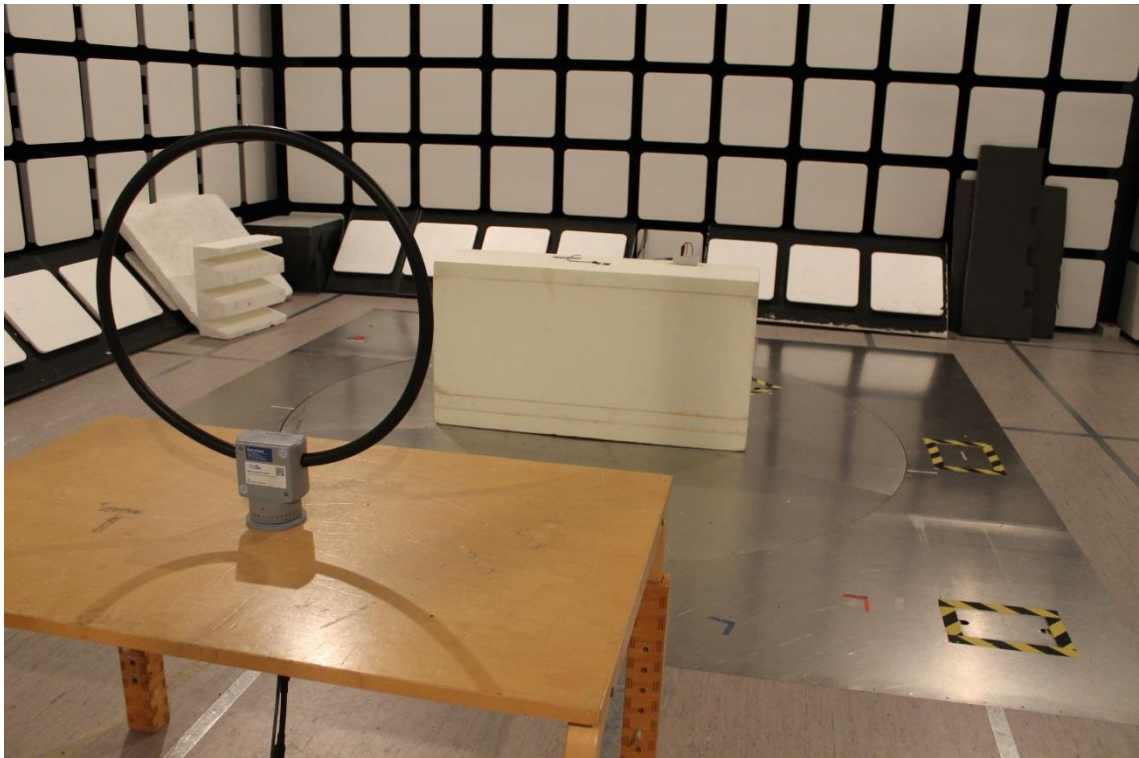
Photograph 2. Radiated Spurious Emissions 9 kHz - 30 MHz
