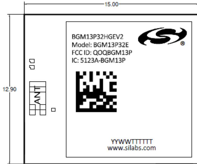
Figure 3: BGM13P32E Label
