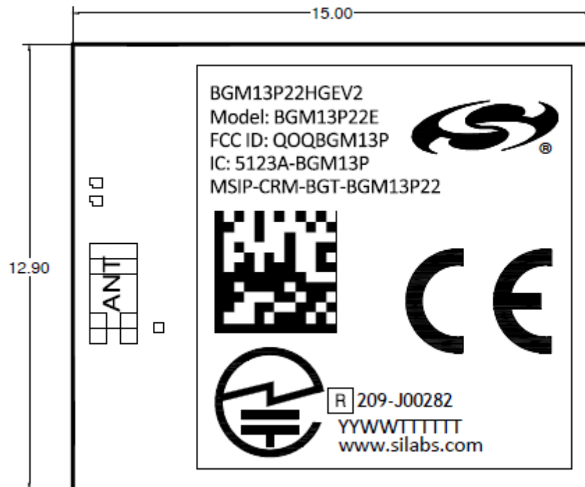
Figure 2: BGM13P22E Label
