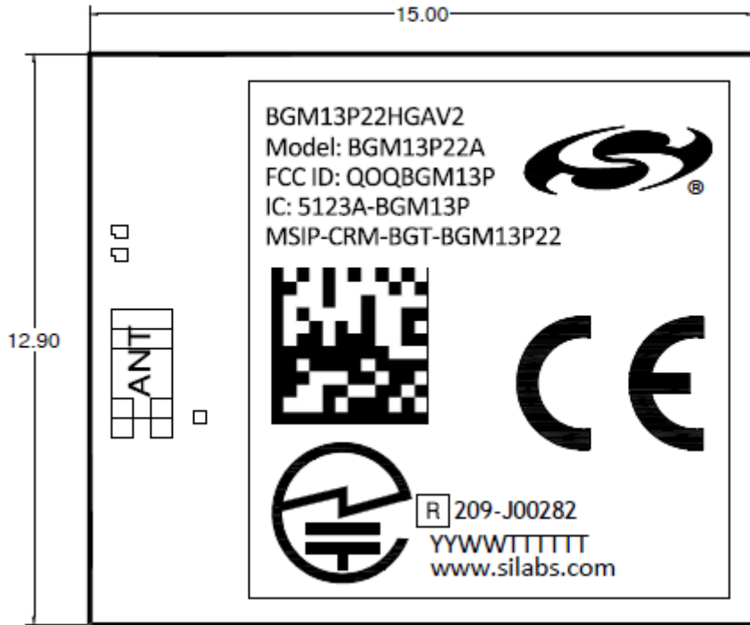
Figure 1: BGM13P22A Label
