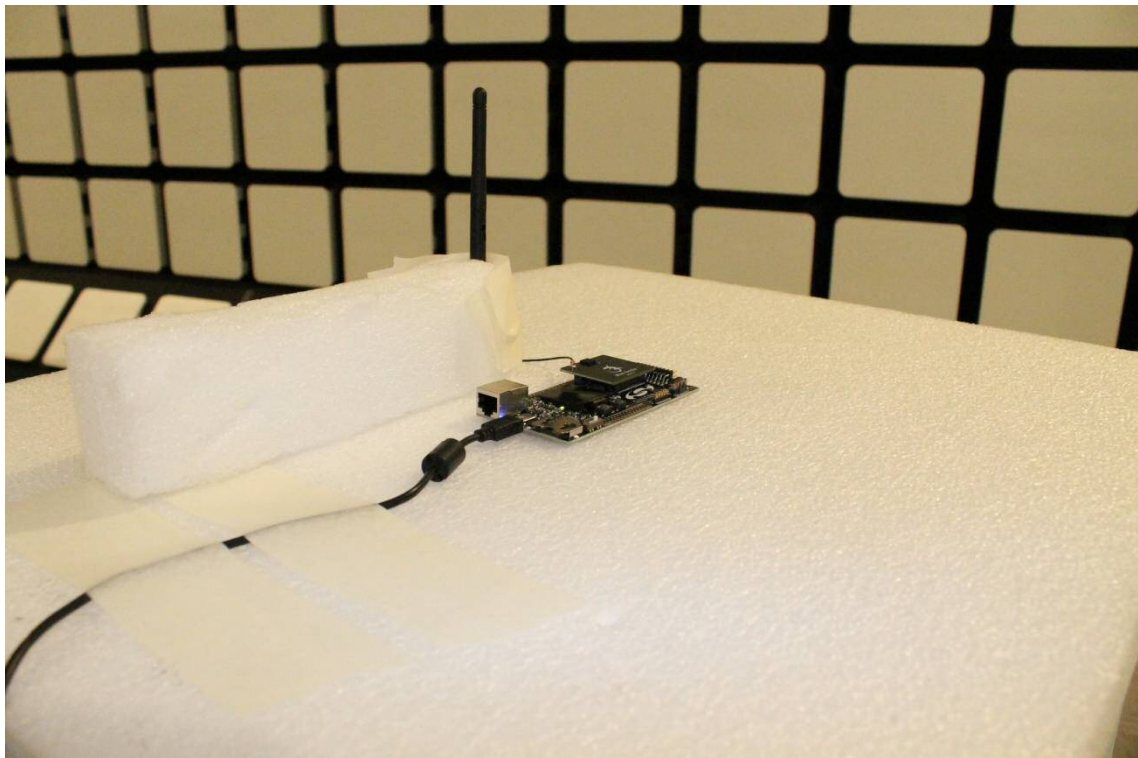
Photograph 4. EUT on table, BGM121N > 1GHz
