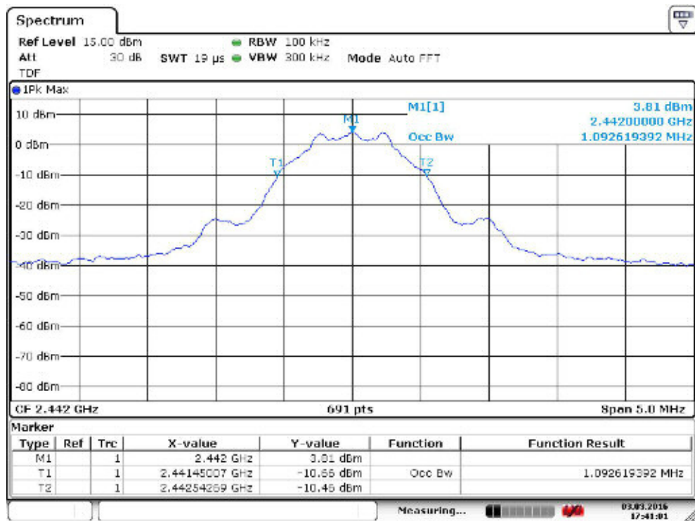
Figure 40. 99 % OBW channel mid.
