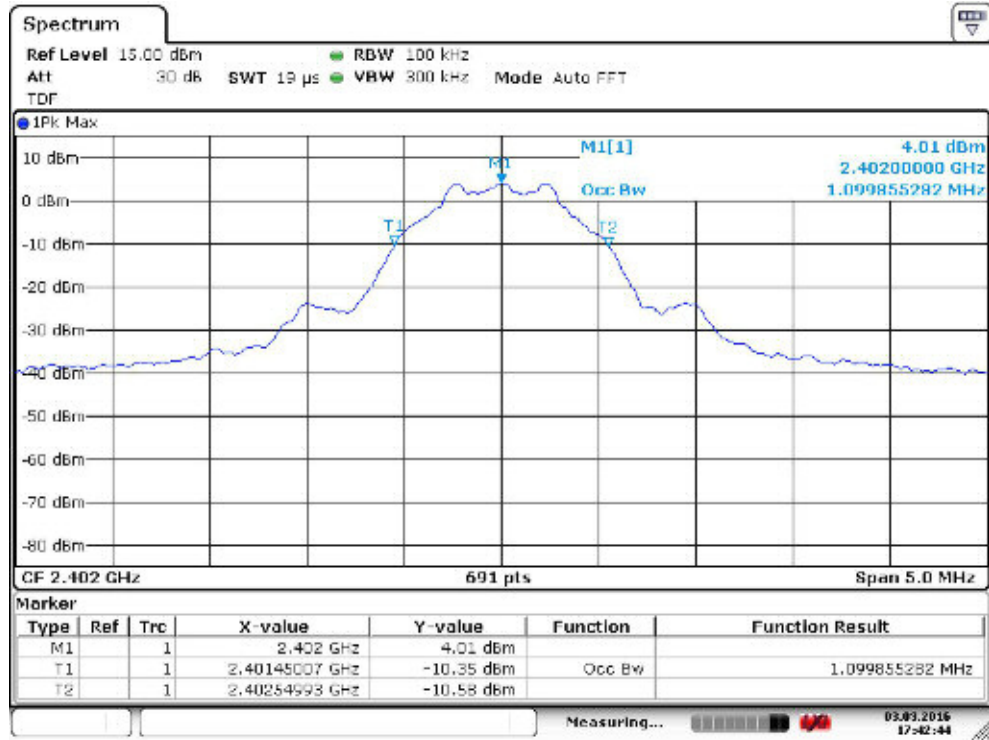
Figure 39. 99 % OBW channel low.
