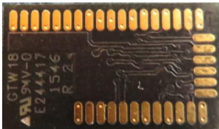
BGM113 BOTTOM
